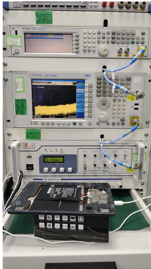
RF Conducted Test Setup Photo
