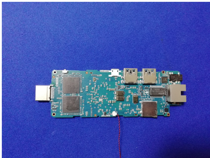
Back view of version A PCB
