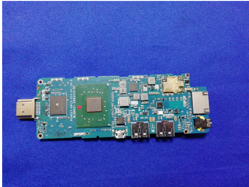
Front view of version A PCB
