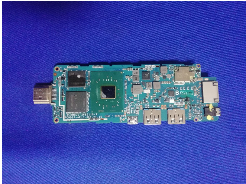
Front view of version B PCB
