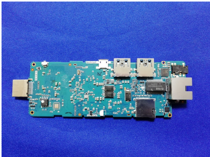
Back view of version B PCB
