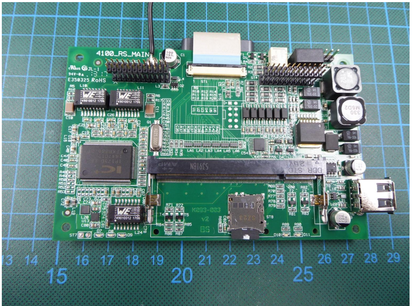
172189_eut15: Top view main PCB without sub PCB
