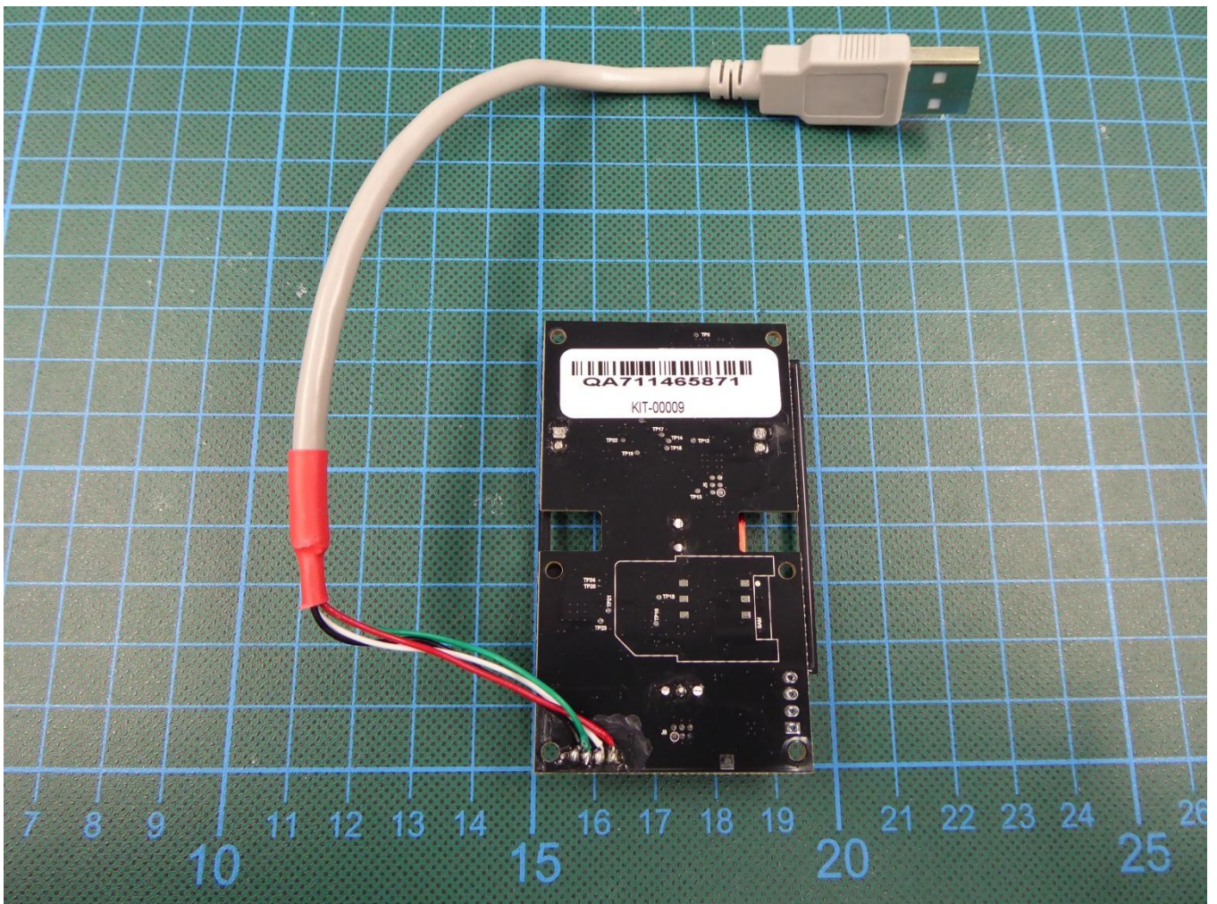
172189_eut23: Bottom view RFID PCB
