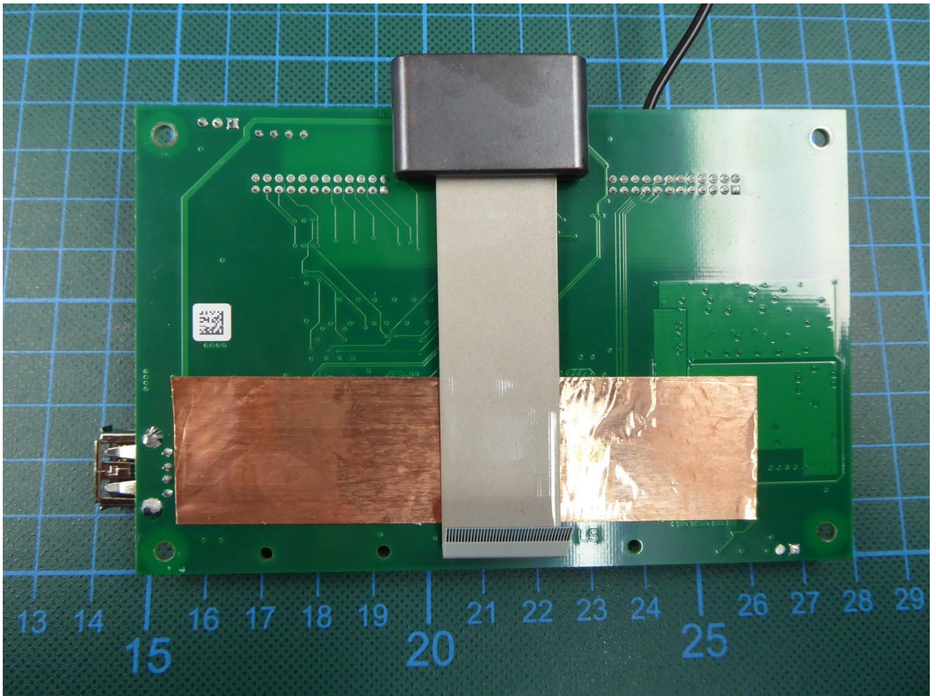
172189_eut12: Bottom view main PCB
