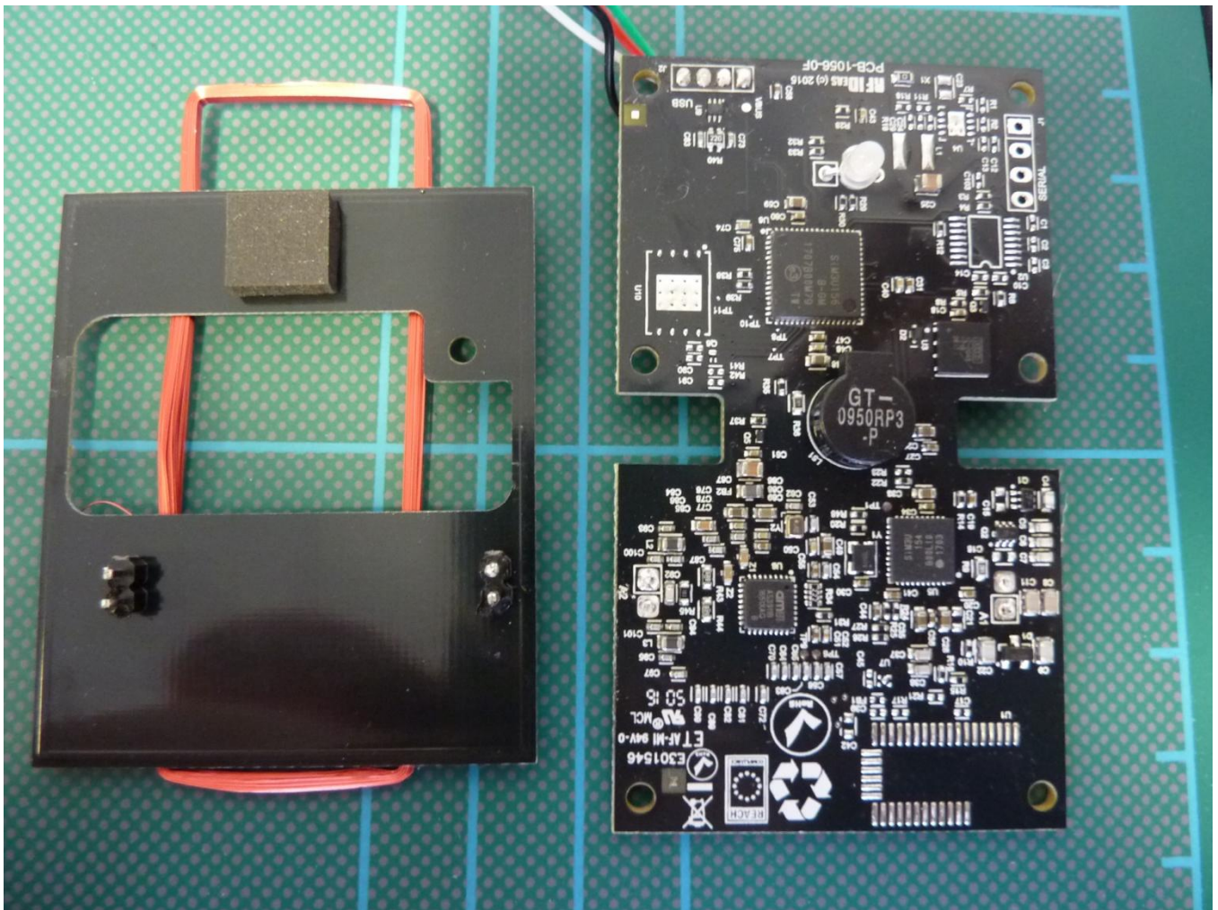
172189_eut25: Bottom view 2 RFID PCB
