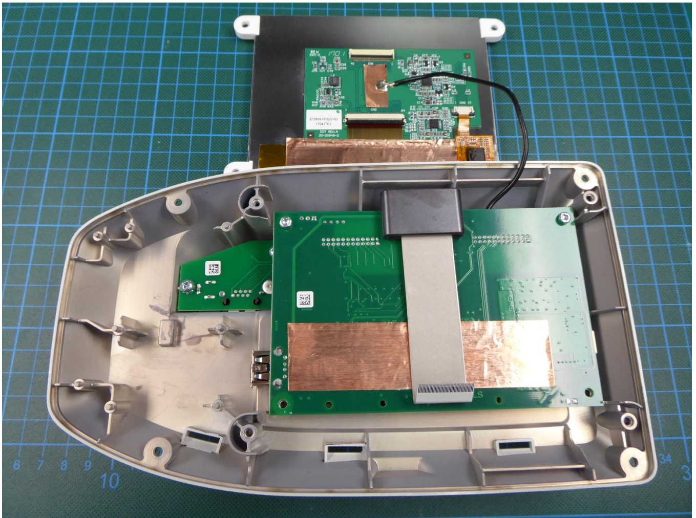
172189_eut10: Internal view 4
