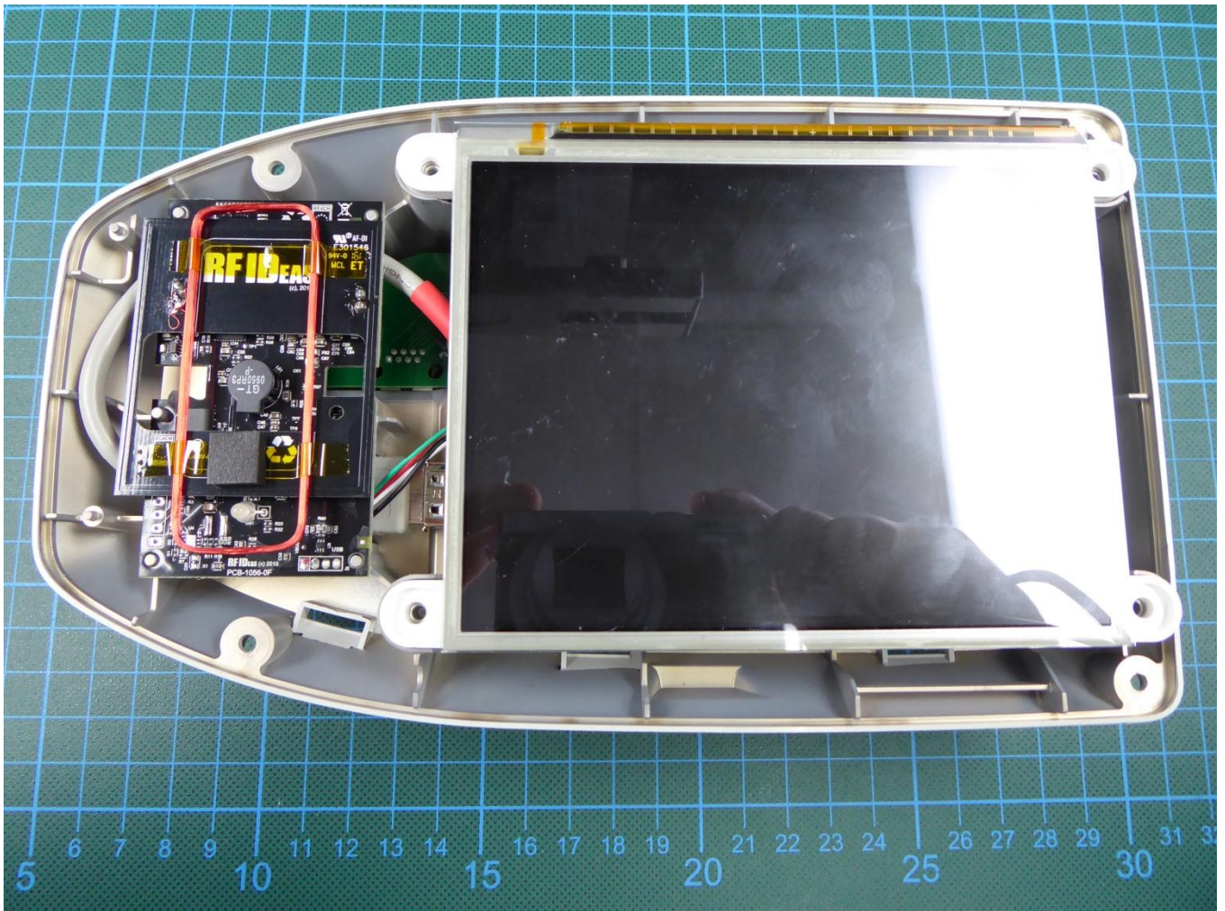
172189_eut8: Internal view 2
