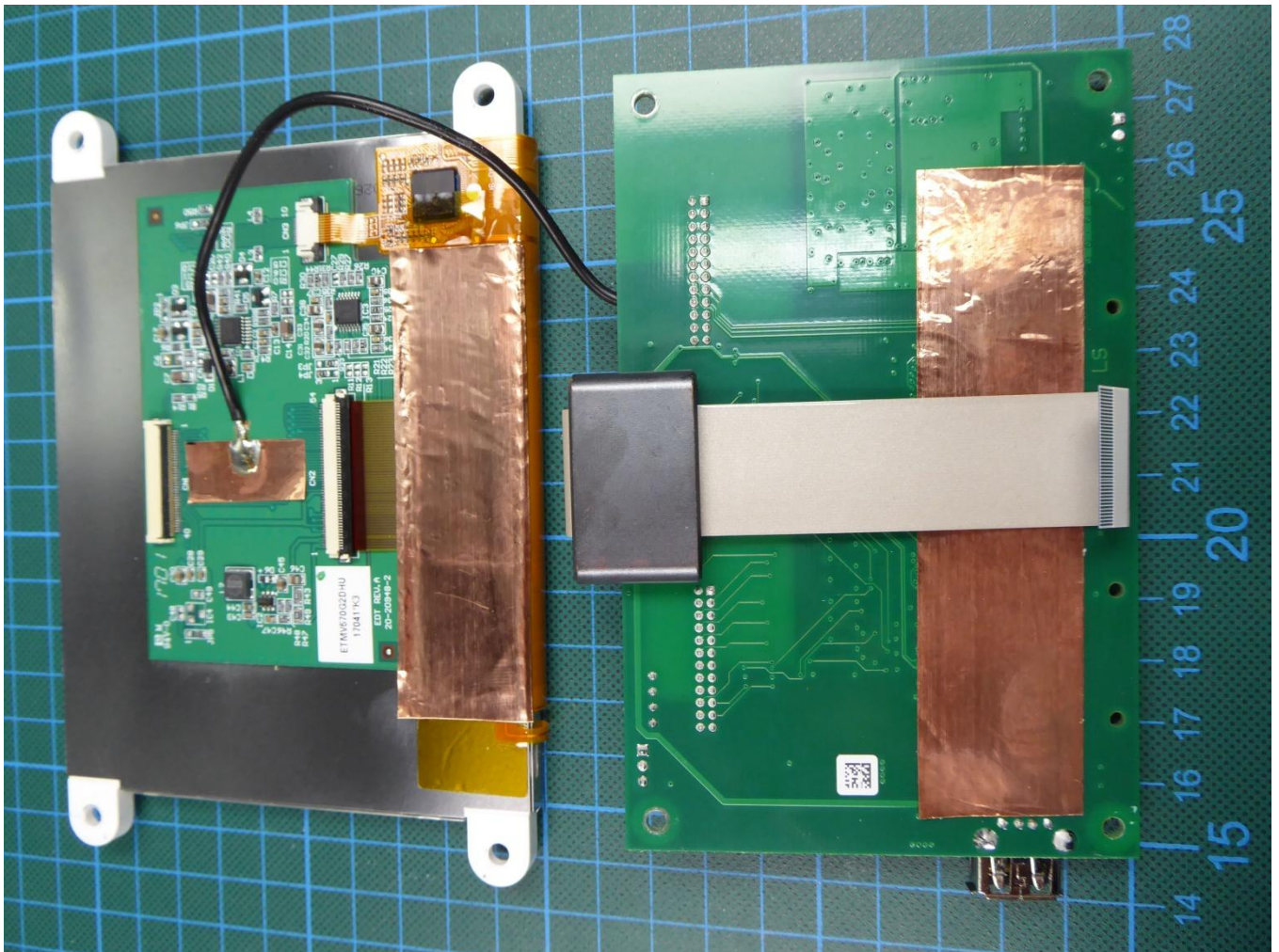
172189_eut11: Bottom view main PCB and Display
