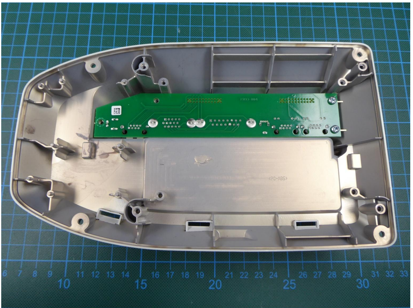
172189_eut18: Internal view 5
