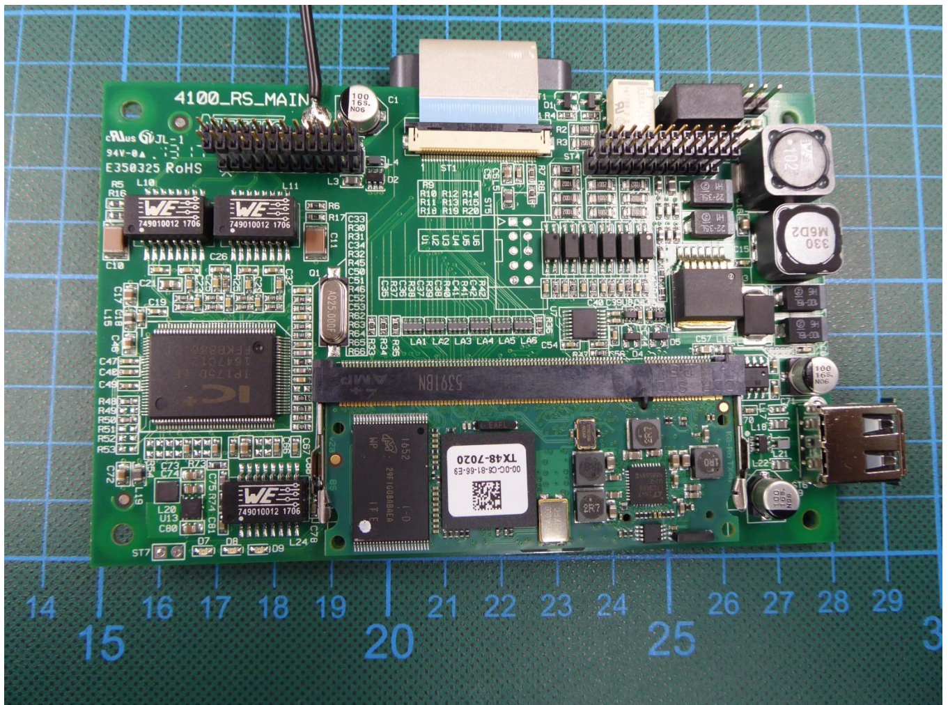
172189_eut14: Top view main PCB with sub PCB
