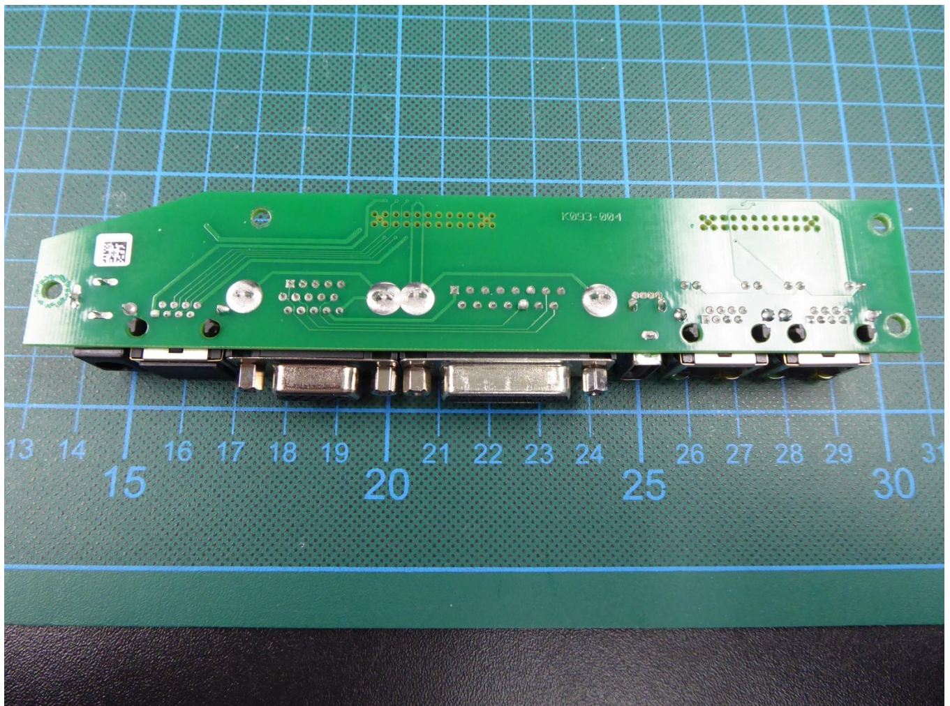
172189_eut20: Bottom view connector PCB
