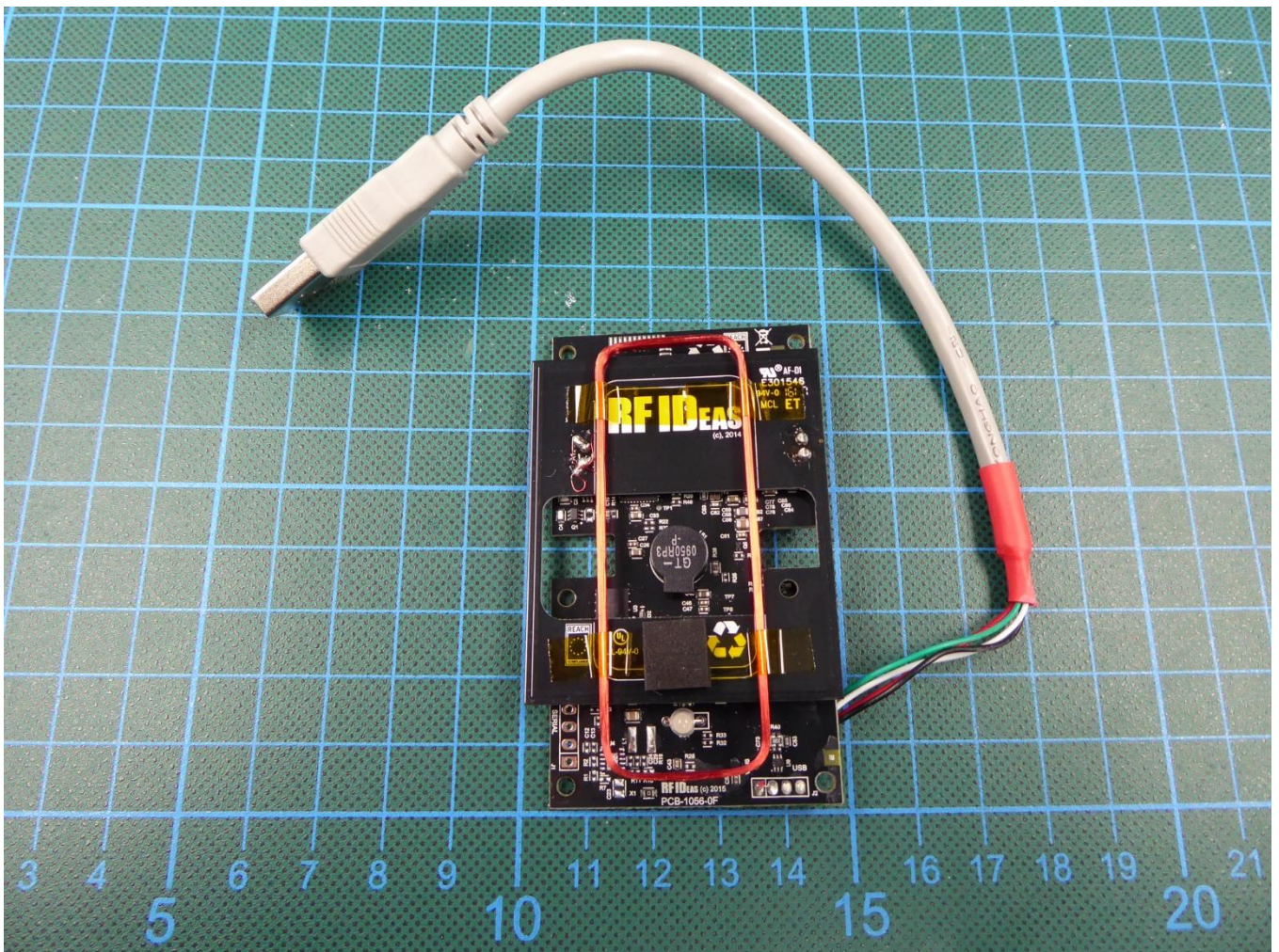
172189_eut22: Top view RFID PCB
