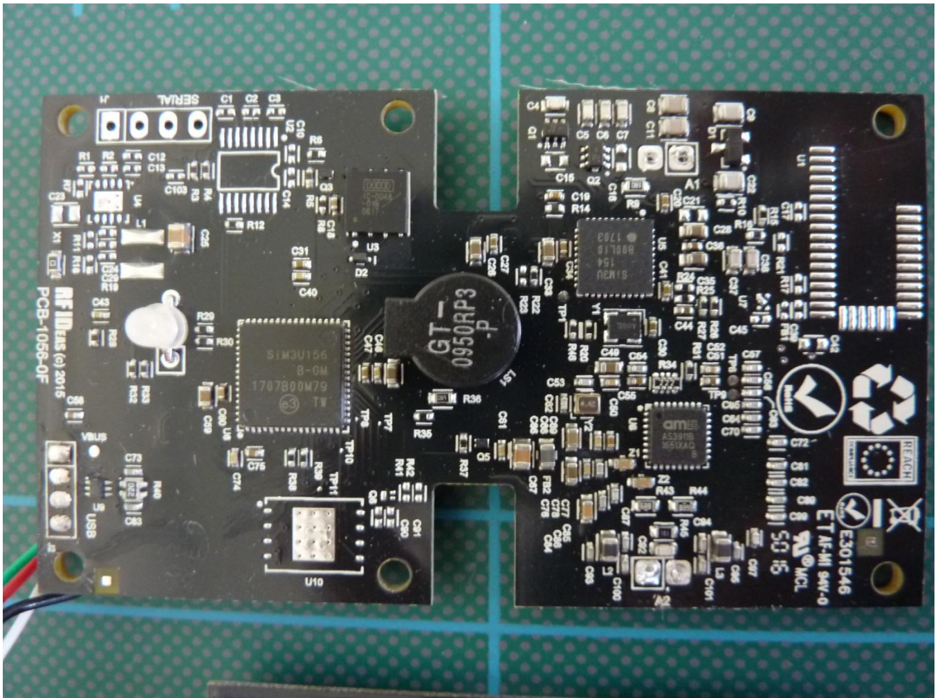
172189_eut26: Detail bottom view RFID PCB
