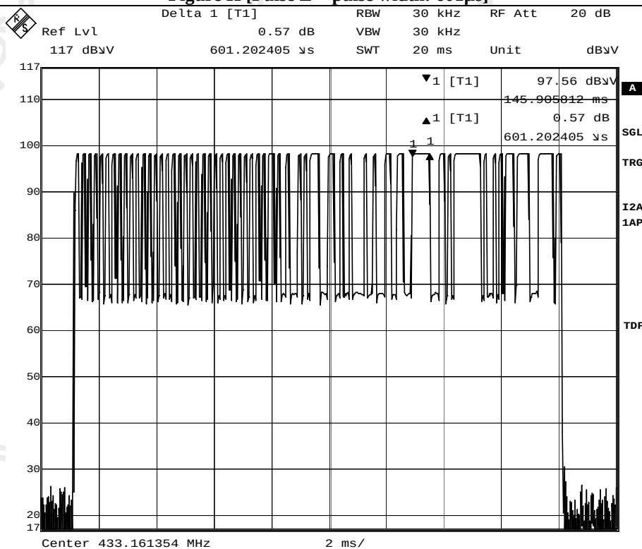
Figure H [Pulse E = pulse width: 601µs]
