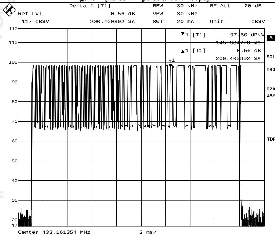
Figure E [Pulse B = pulse width: 200 \mu s]
