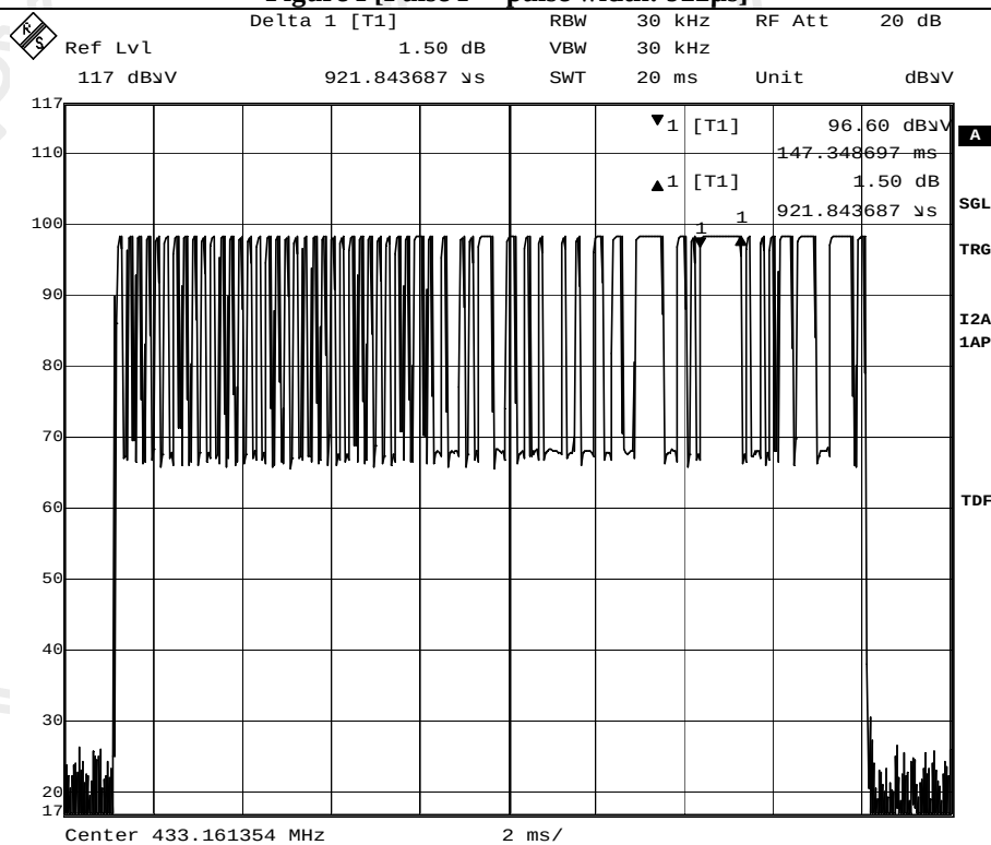
Figure I [Pulse F = pulse width: 922µs]
