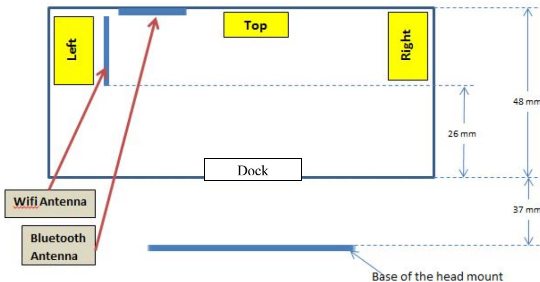
Figure-1 Head Parallel Mount Top View
