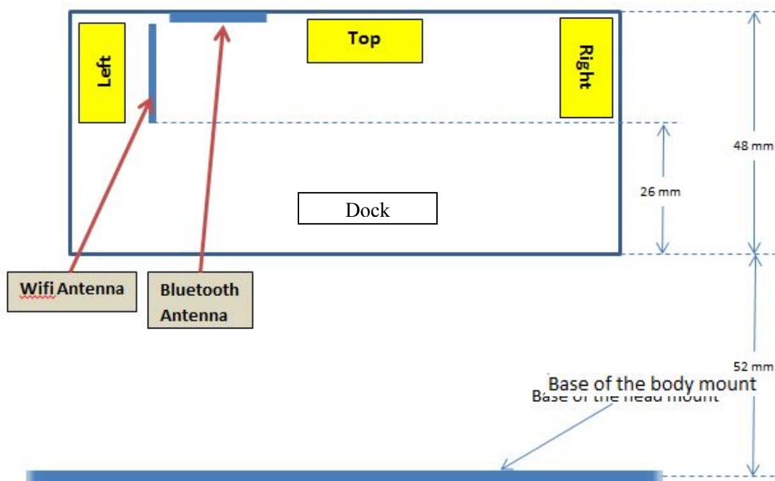
Figure-4 Body Vertical Mount Back View
