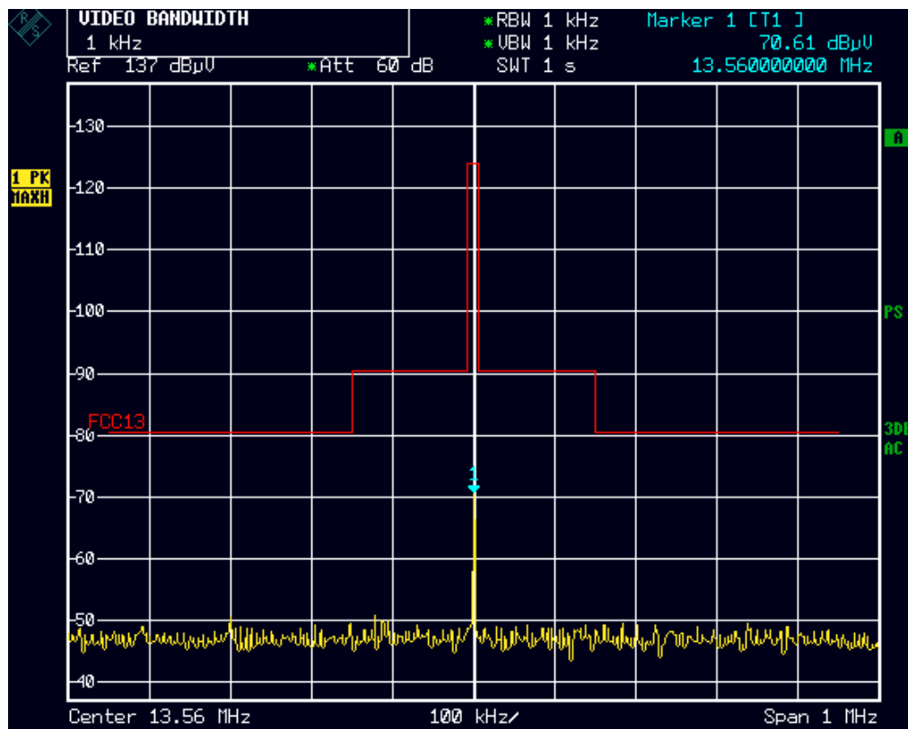
Figure 4: Spectrum Mask
