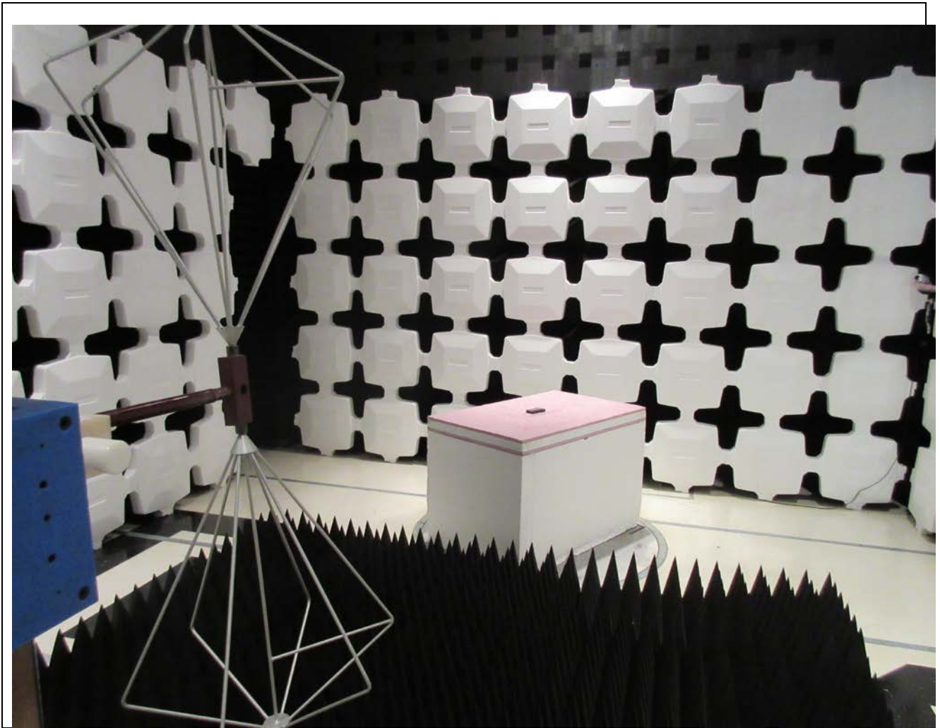
RADIATED EMISSIONS TEST SET UP PHOTO
