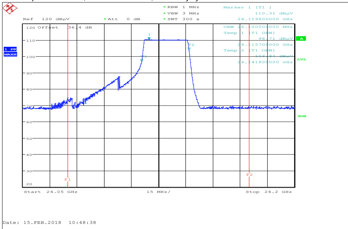
Plot 14: Occupied bandwidth, 30 MHz bandwidth, 10 % duty cycle
