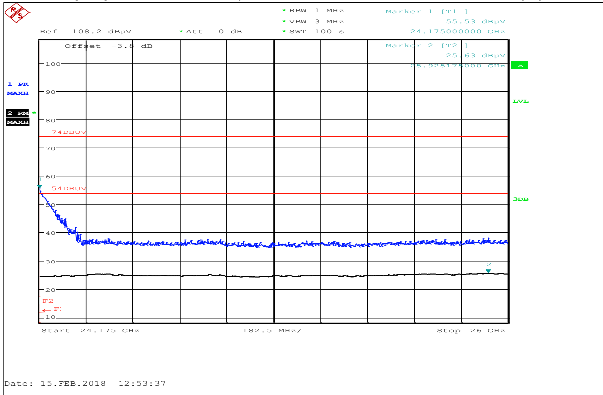
Plot 21: Band edge high, horizontal / vertical polarization, valid for all modulation and both duty cycle
