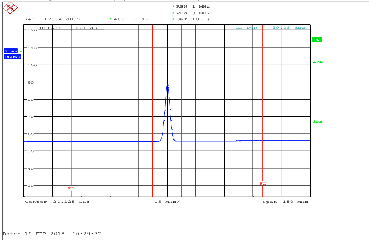
Plot 2: Field strength, CW, 10 % duty cycle, Detector Average
