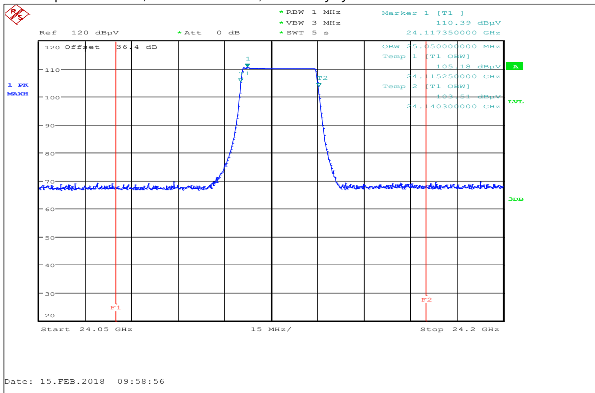
Plot 15: Occupied bandwidth, 30 MHz bandwidth, 100 % duty cycle
