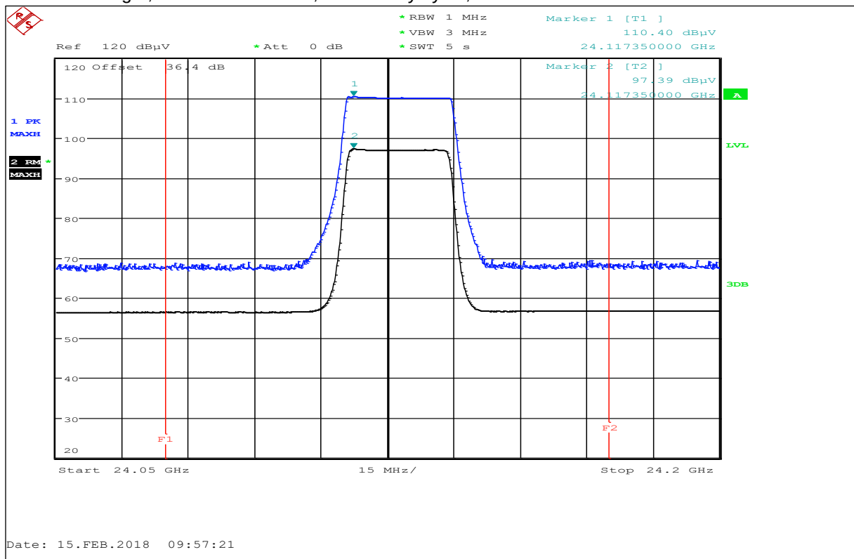
Plot 10: Field strength, 30 MHz bandwidth, 100 % duty cycle, Detector Peak / RMS
