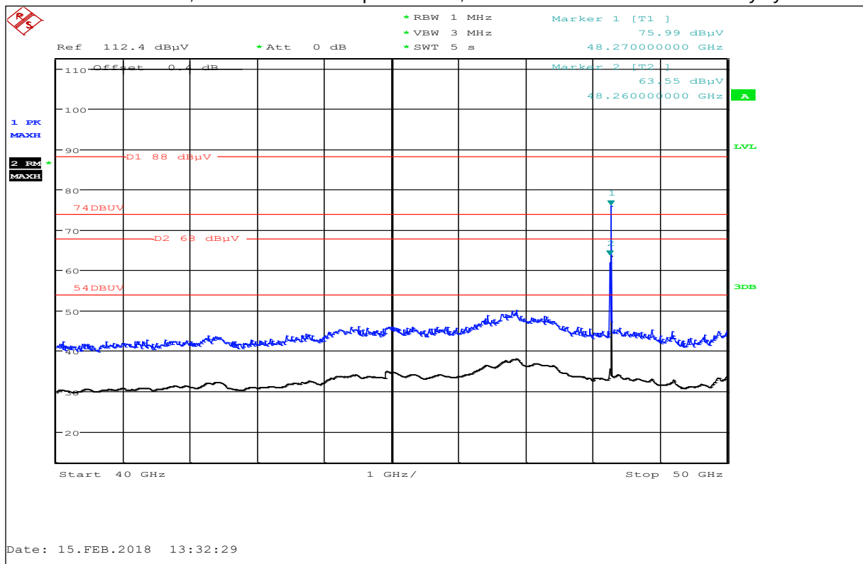
Plot 27: 40 GHz to 50 GHz, horizontal / vertical polarization, 10 MHz bandwidth and 100% duty cycle
