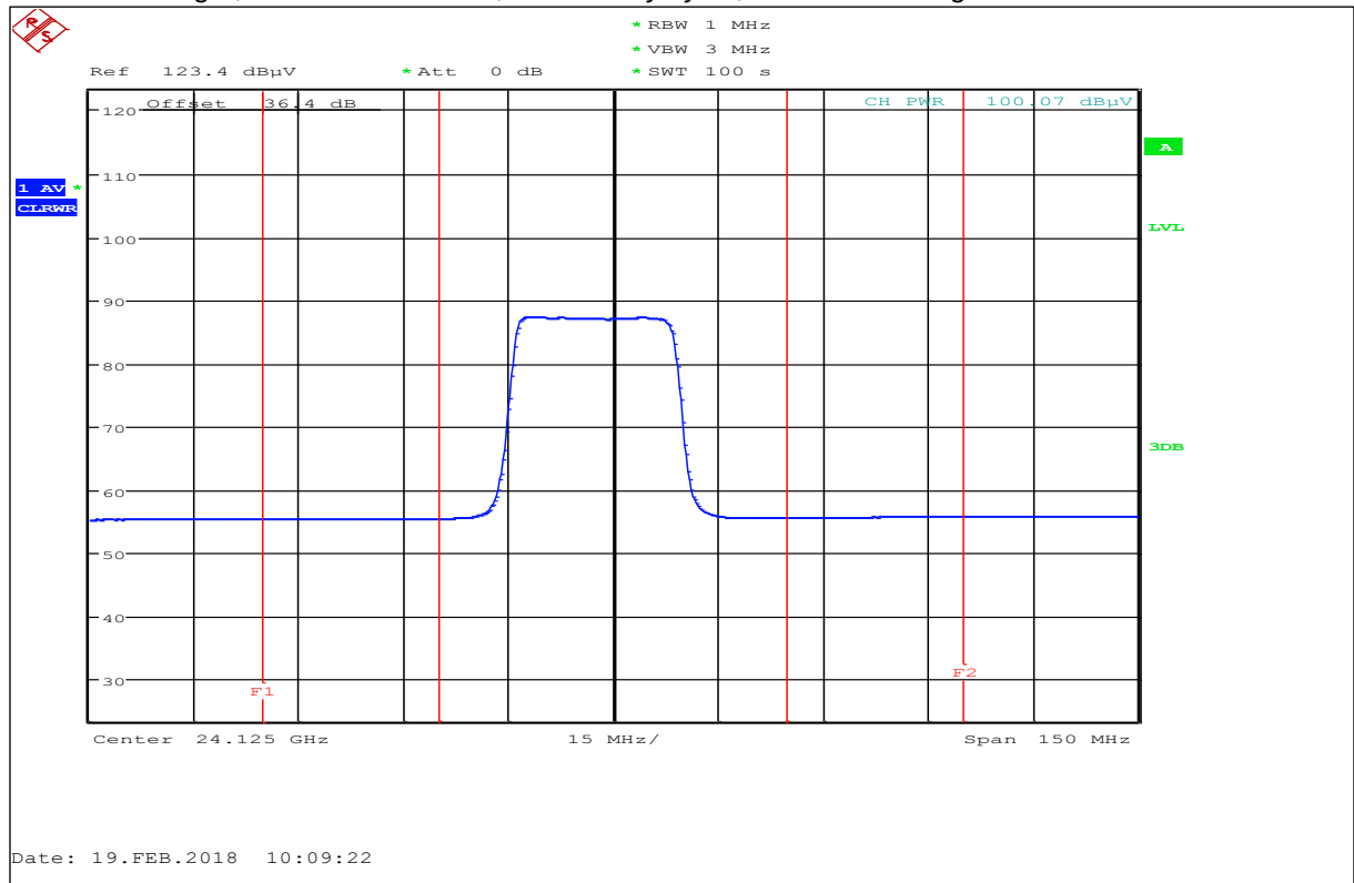
Plot 11: Field strength, 30 MHz bandwidth, 100 % duty cycle, Detector Average
