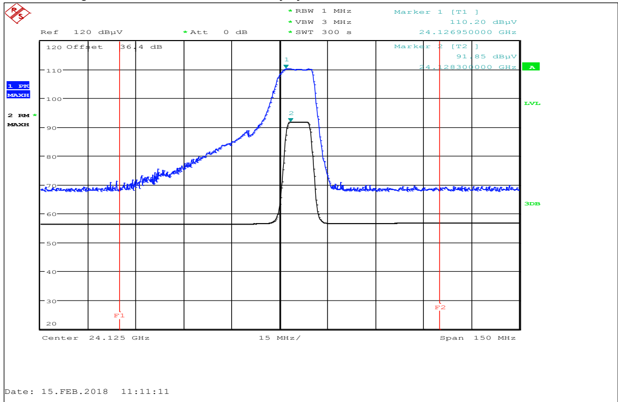
Plot 4: Field strength, 10 MHz bandwidth, 10 % duty cycle, Detector Peak / RMS
