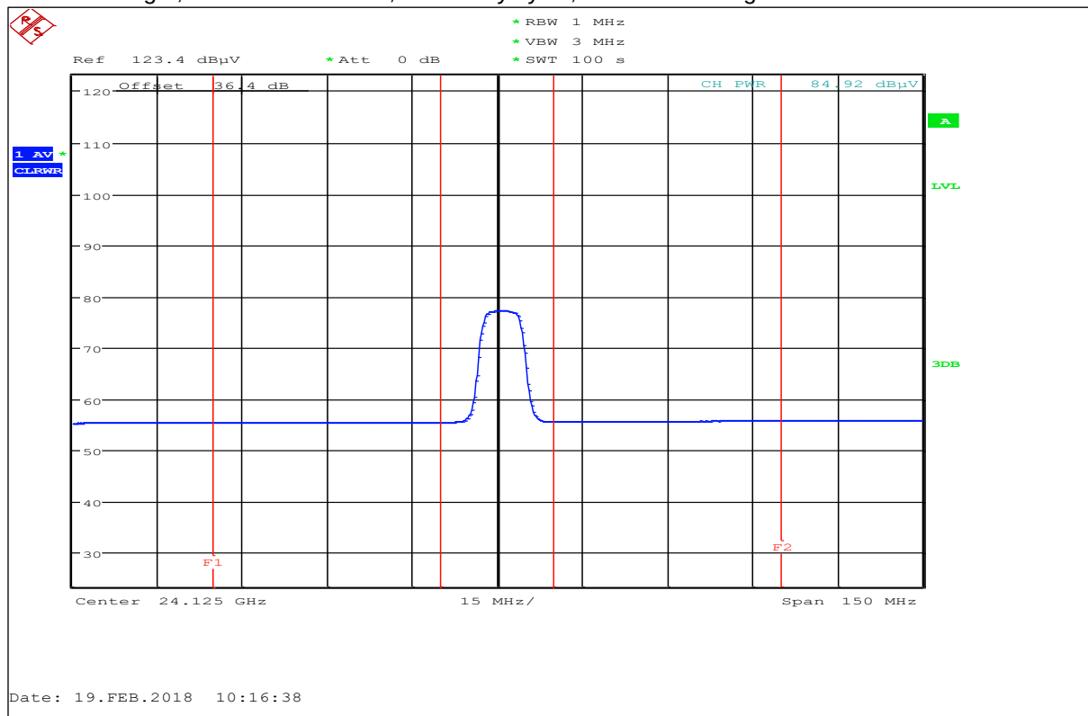
Plot 5: Field strength, 10 MHz bandwidth, 10 % duty cycle, Detector Average
