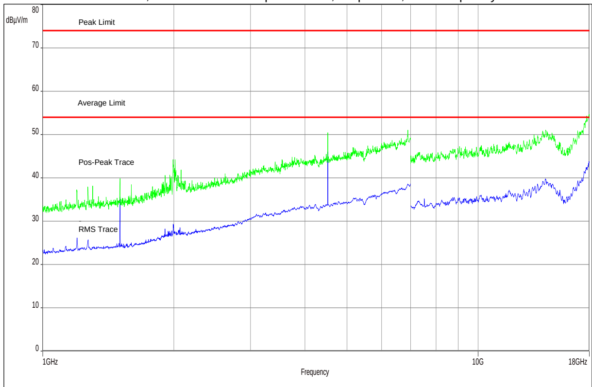
Plot No. 11: 1 GHz to 18 GHz, horizontal / vertical polarization, Stop Mode, Low Frequency
