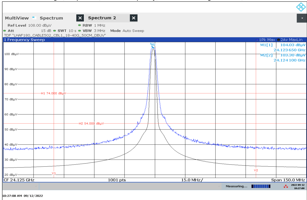
Plot No. 3: Field Strength, Stop Mode, Middle Frequency, Peak and Average detector, T_{\text{nom}} / V_{\text{nom}}
