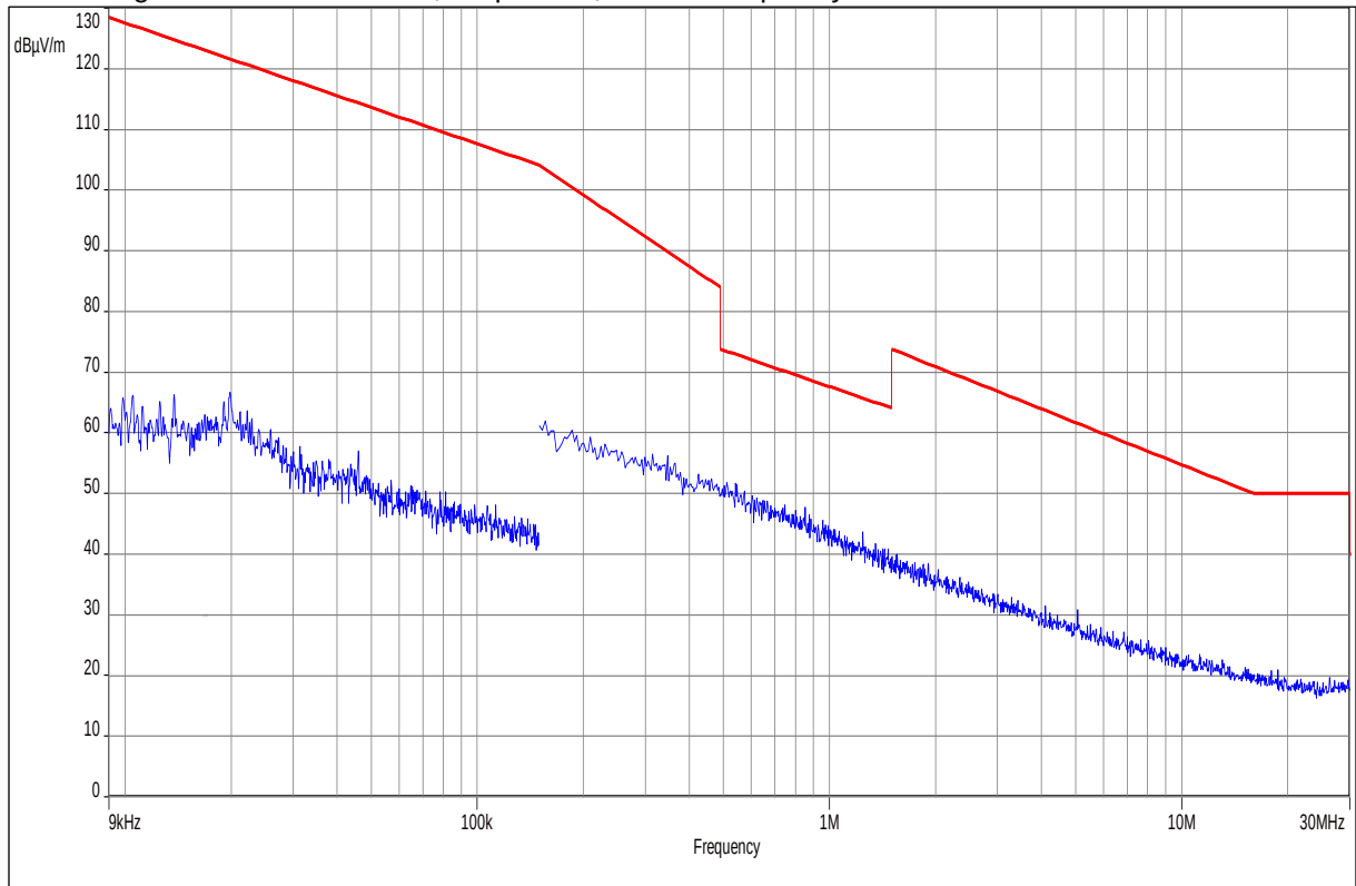
Plot No. 7: Magnetic: 9 kHz - 30 MHz, Stop Mode, Middle Frequency
