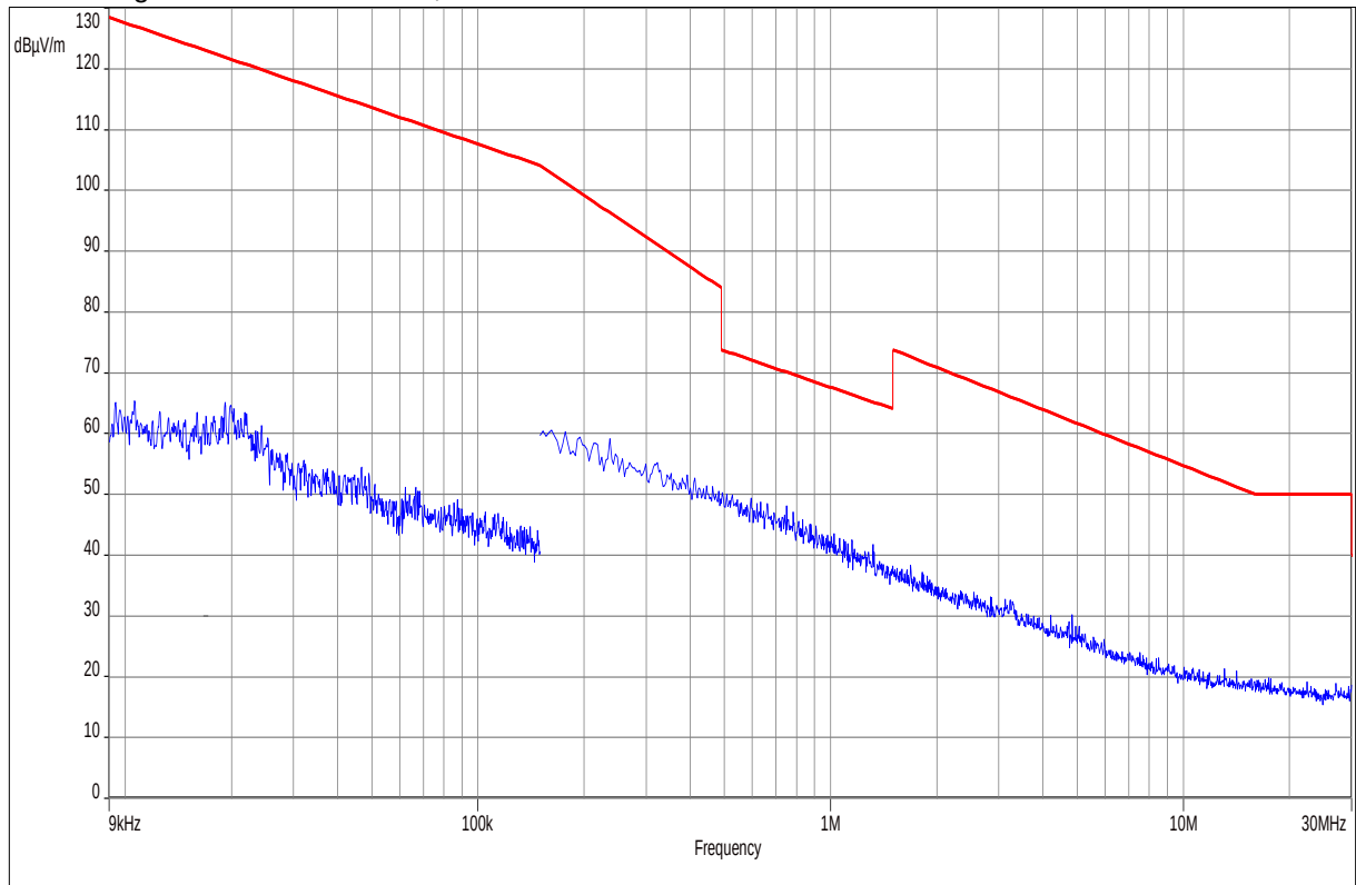
Plot No. 5: Magnetic: 9 kHz - 30 MHz, Normal Mode
