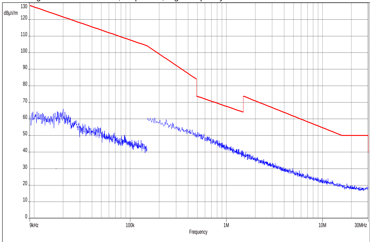
Plot No. 8: Magnetic: 9 kHz - 30 MHz, Stop Mode, High Frequency
