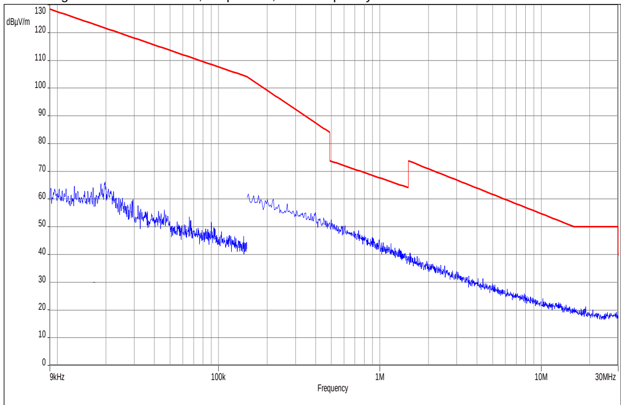
Plot No. 6: Magnetic: 9 kHz - 30 MHz, Stop Mode, Low Frequency
