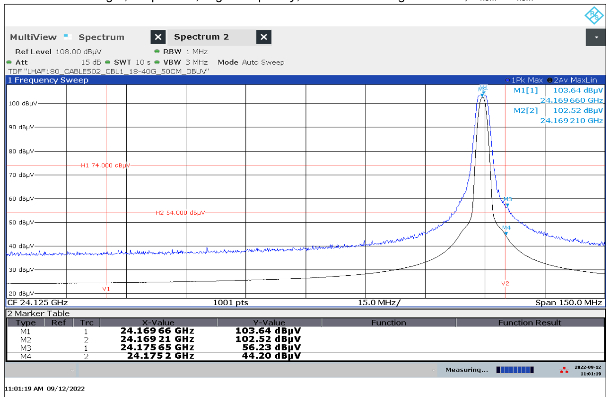
Plot No. 4: Field Strength, Stop Mode, High Frequency, Peak and Average detector, T_{\text{nom}} / V_{\text{nom}}
