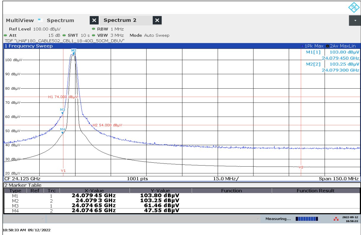
Plot No. 16: Band Edge Low, horizontal / vertical polarization
