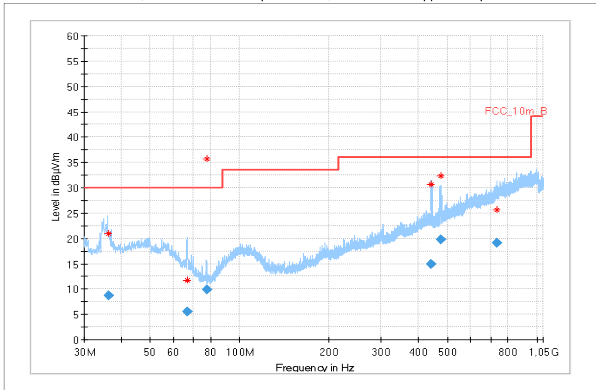
Plot No. 9: 30 MHz to 1 GHz, horizontal / vertical polarization, Valid for all Stopped Frequencies
