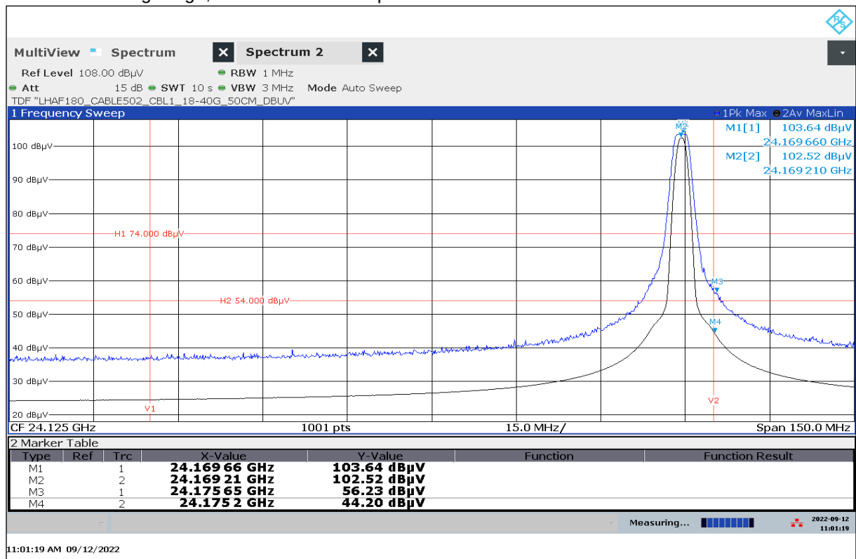
Plot No. 17: Band Edge High, horizontal / vertical polarization
