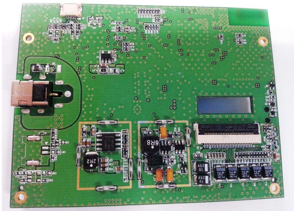
Main Board-Rear
