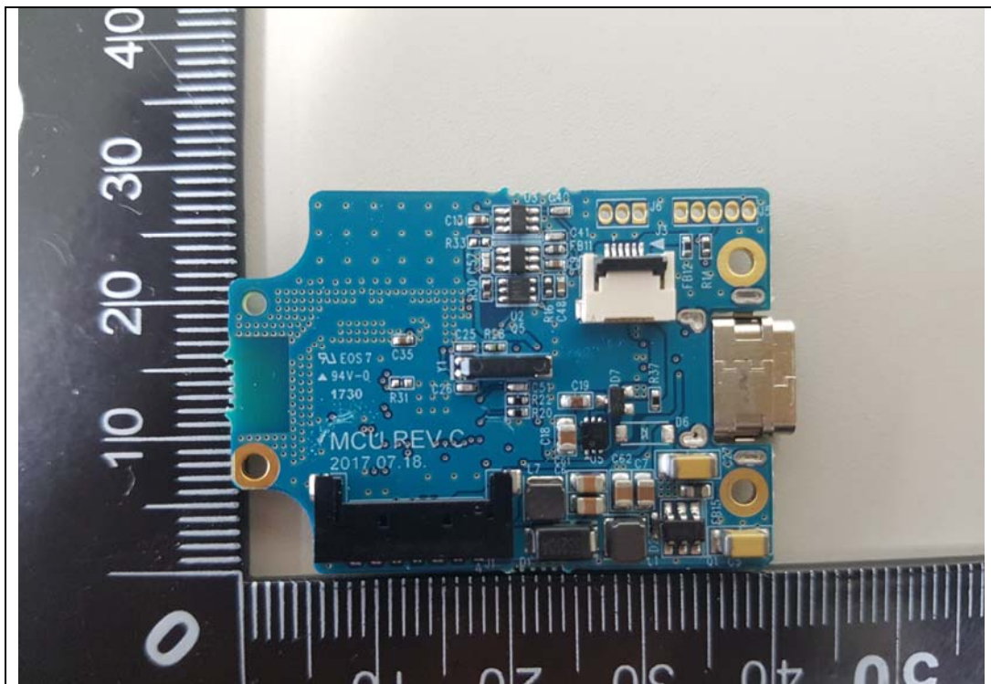
MCU Board Rear
