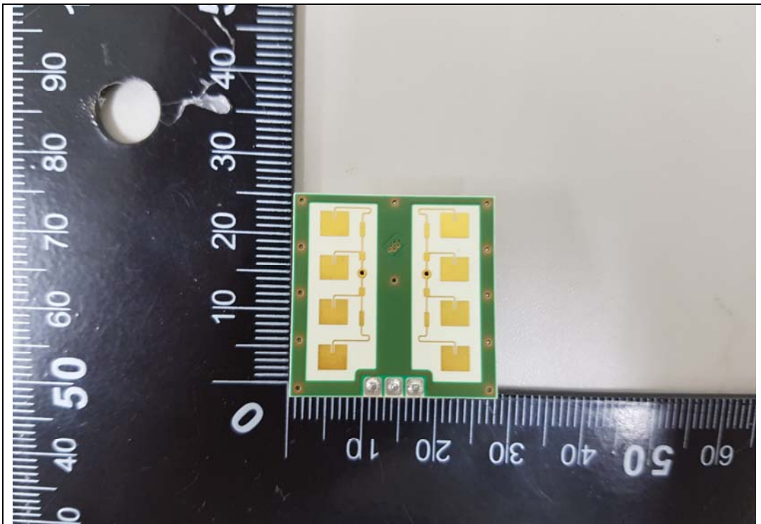
Radar Module Rear
