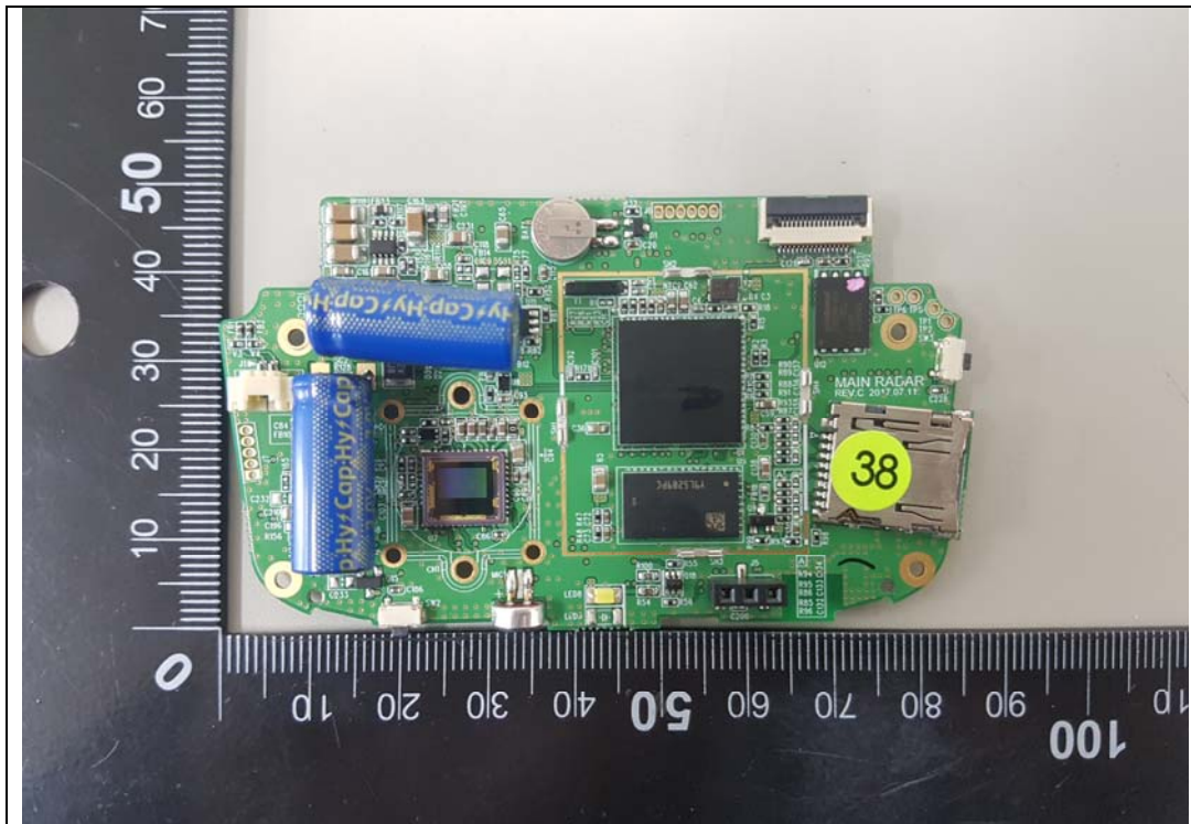
Main Radar Board Front
