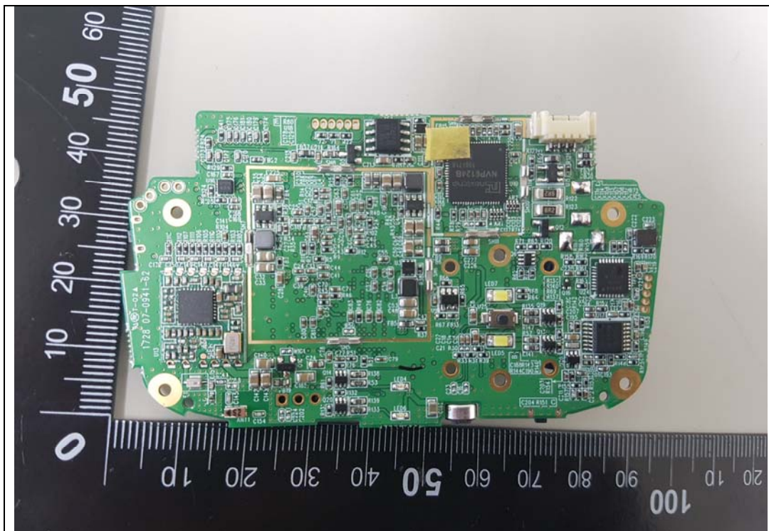
Main Radar Board Rear
