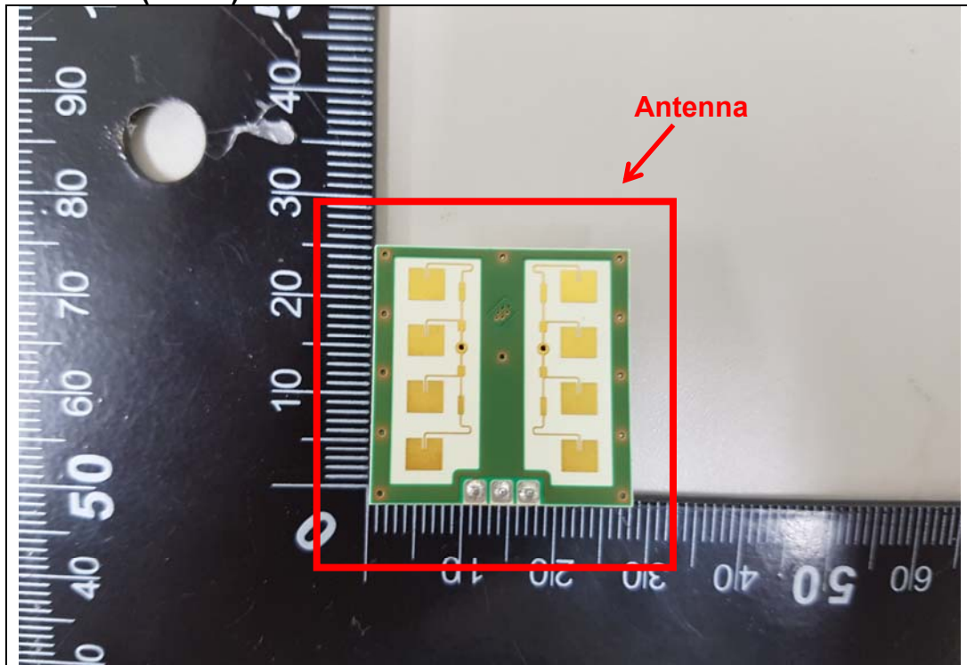
Antenna (Radar)
