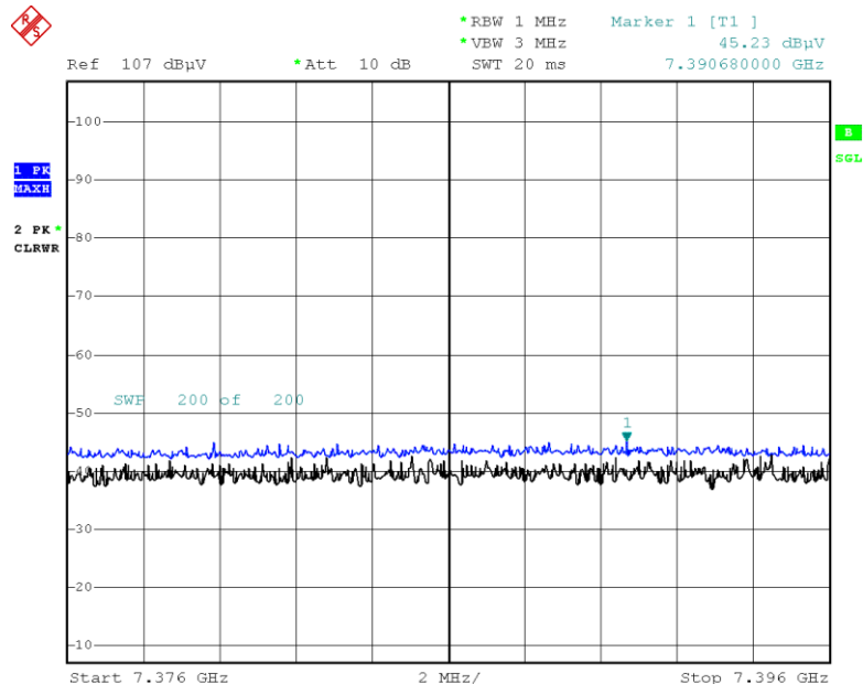
Radiated Spurious Emissions plot – Peak Reading (802.11n, Ch.11 3rd Harmonic)
