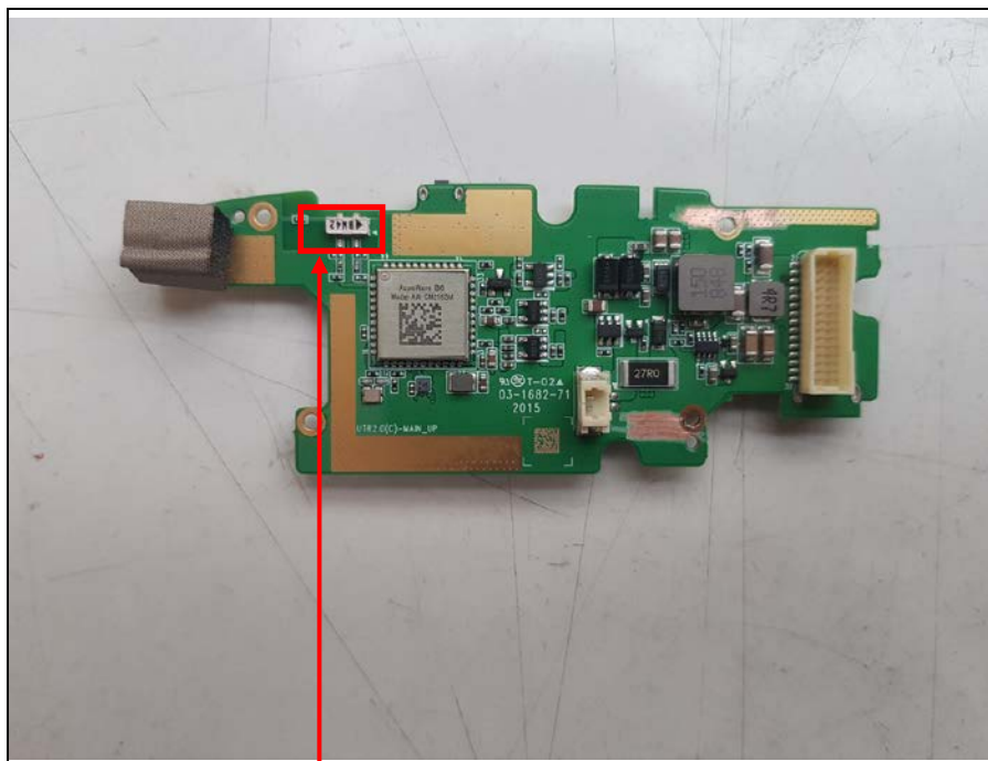
WLAN Antenna
