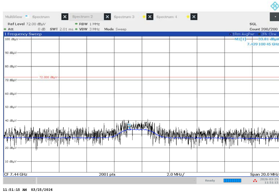
Radiated Spurious Emissions plot – Average Result (Ch.39 3rd Harmonic)
