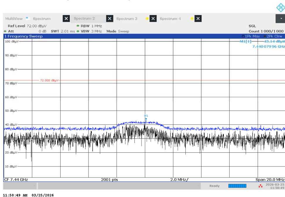
Radiated Spurious Emissions plot – Peak Result (Ch.39 3rd Harmonic)
