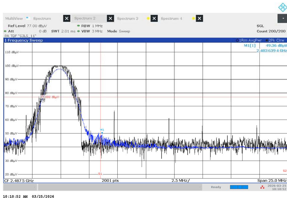
Radiated Restricted Band Edges plot – Average Result (Ch.39, Y-V)
