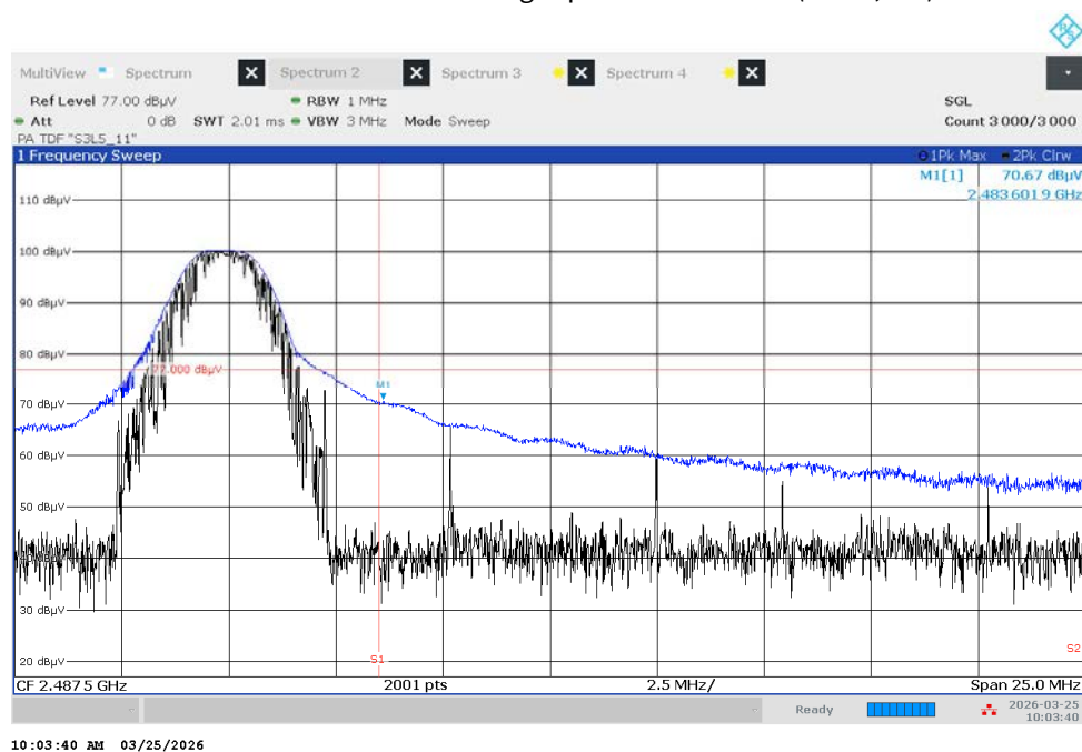
Radiated Restricted Band Edges plot – Peak Result (Ch.39, Y-V)
