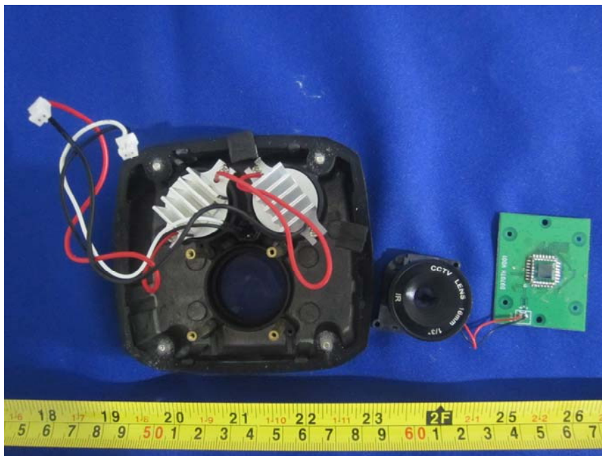
EUT – Camera Board Off View
