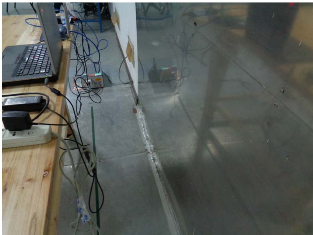
Conducted Emissions Setup Side View
