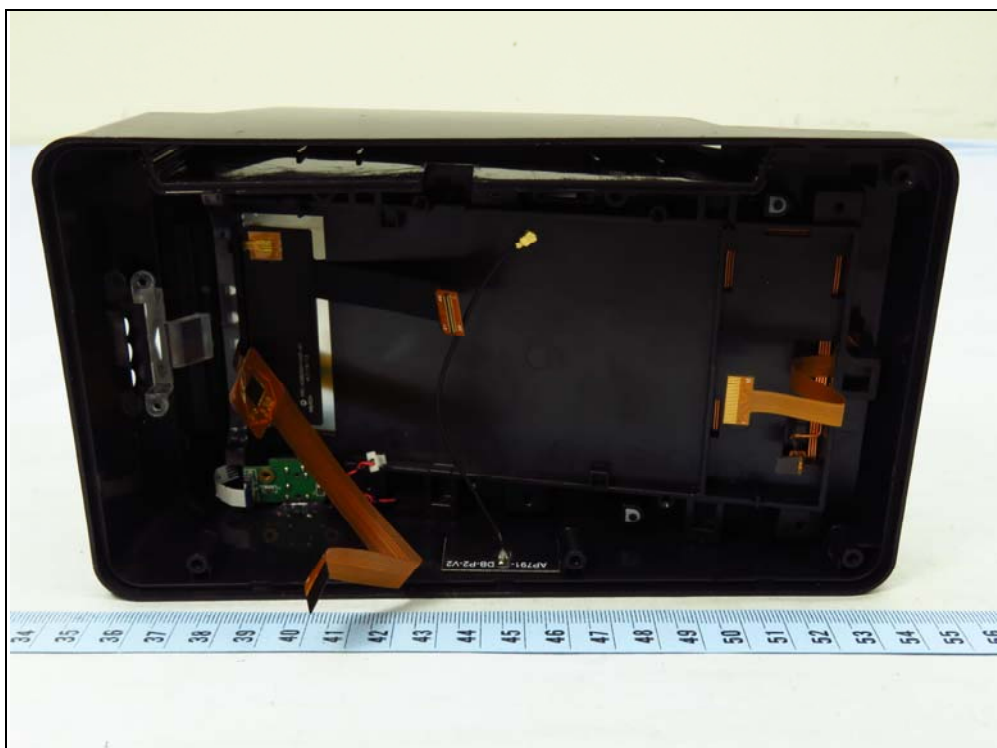
BT/WLAN antenna
