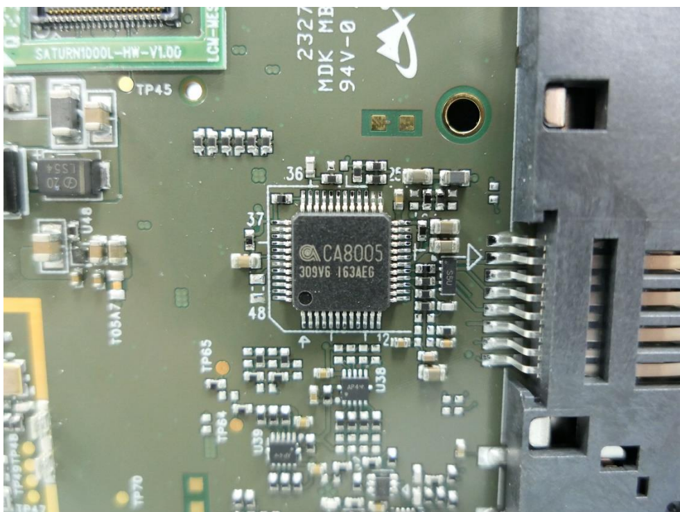
(38) EUT Photo
