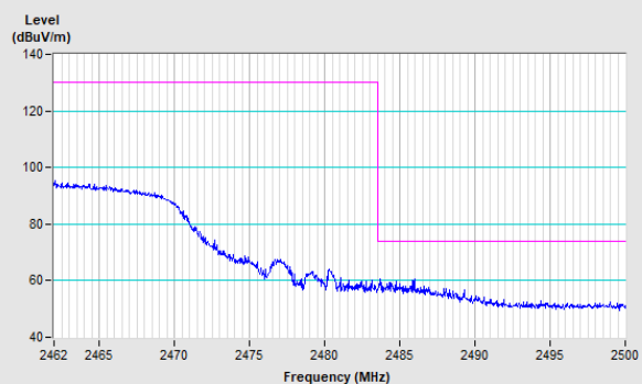
Horizontal (Peak)
