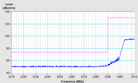
Vertical (Peak)
