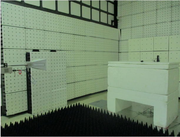
LTE_Radiated_Setup
