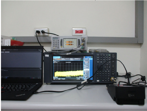
BLE_Conducted_Setup
