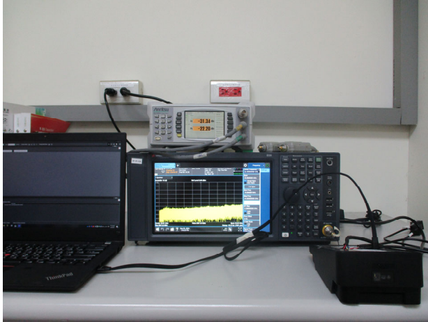
WLAN_2.4G_Conducted_Setup
