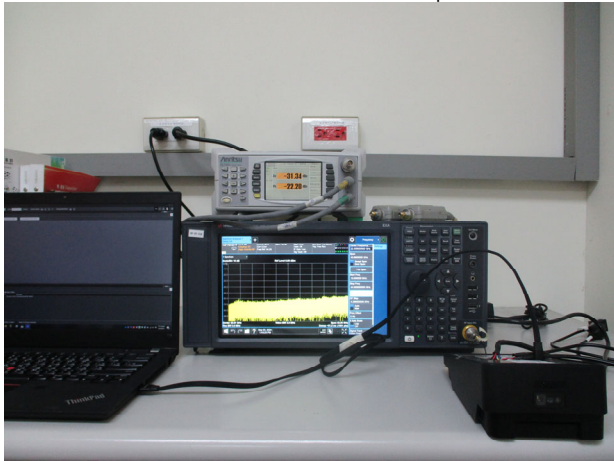
WLAN_2.4G_Conducted_Setup
