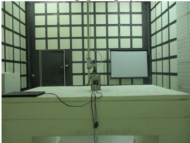
2G_3G_Radiated_Setup
