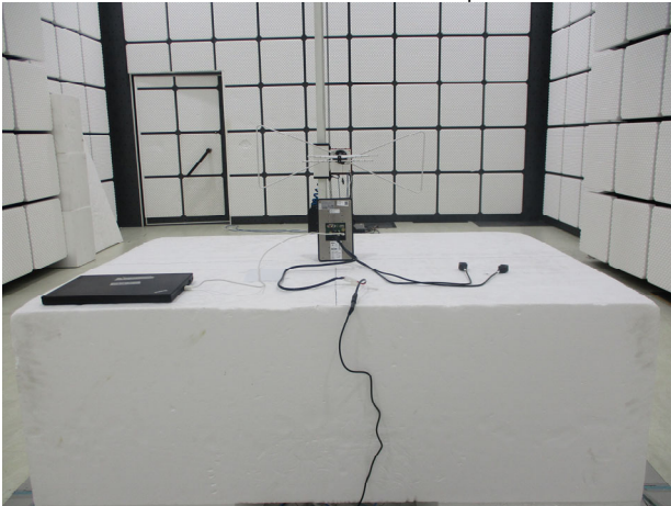
WLAN 2.4G_Radiated_Setup
