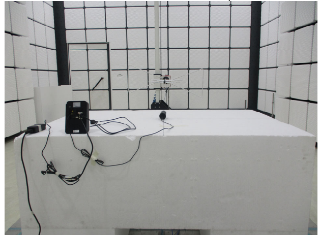
FCC_24_E_4G_Radiated_Setup
