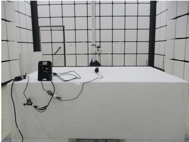
FCC_22_H_2G_Radiated_Setup
