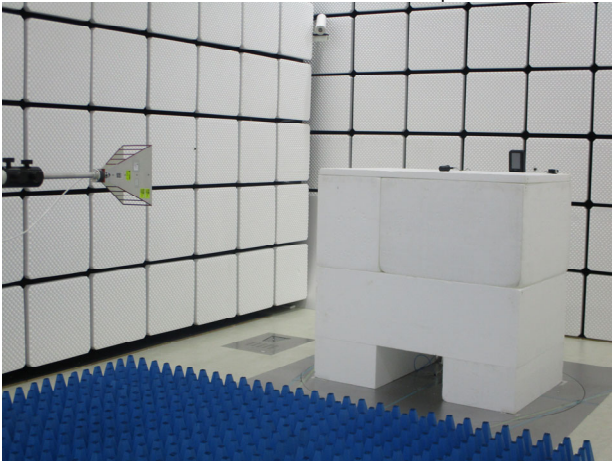
FCC_24_E_4G_Radiated_Setup
