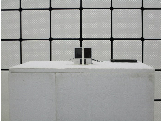
Part_15_247+RSS-247_BT_Radiated_Setup
