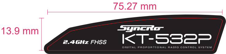
B-TKYGT2EB532P-01 KY-GT2EB(532P)底座贴-左 0.25磨砂PC+513胶 75.27*13.9mm
