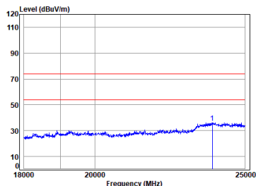
BLE_2M_TX_CH_19_Horizontal
