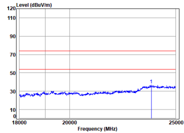
BLE_1M_TX_CH_00_Vertical
