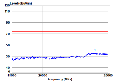
BLE_1M_TX_CH_19_Vertical
