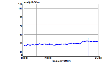
BLE_1M_TX_CH_00_Horizontal
