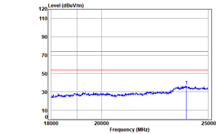
BLE_1M_TX_CH_19_Horizontal
