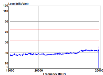
BLE_2M_TX_CH_19_Vertical
