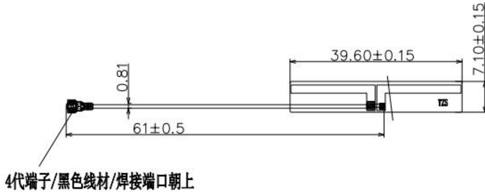
Figure 1 ABB0301 antenna
