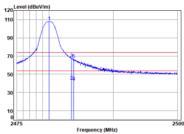
BT_DH5_TX_CH_78_Horizontal
