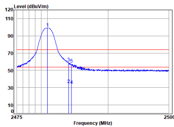
BT_DH5_TX_CH_78_Vertical
