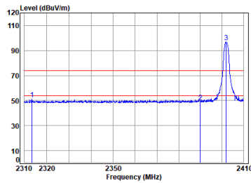
BT_DH5_TX_CH_00_Vertical
