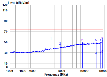
BT_DH5_TX_CH_00_Horizantal
