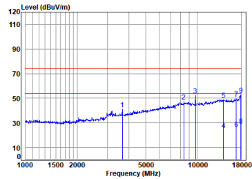
BT_DH5_TX_CH_39_Vertical
