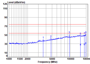
BT_DH5_TX_CH_00_Vertical
