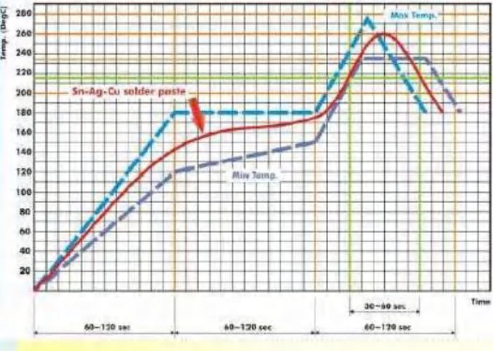
Fig 2.Infrared soldering profile
