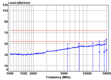
BT_3DH5_TX_CH_00_Horizontal
