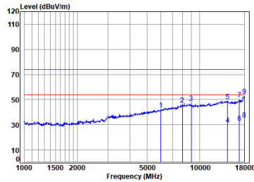
BT_3DH5_TX_CH_78_Horizontal
