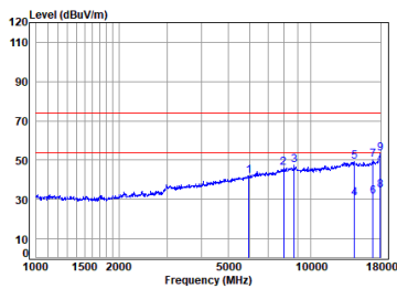
BT_3DH5_TX_CH_39_Horizontal
