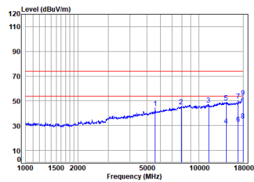
BT_3DH5_TX_CH_39_Vertical
