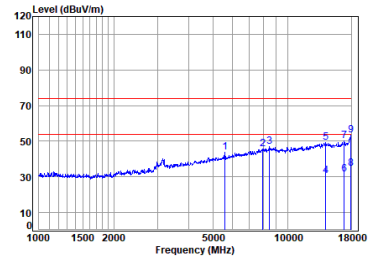
BT_3DH5_TX_CH_78_Vertical
