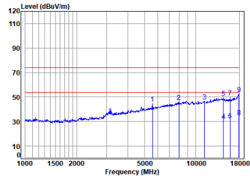
BT_3DH5_TX_CH_00_Vertical
