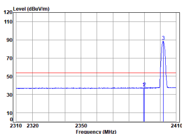
BLE_1M_TX_CH_00_Vertical-AVG
