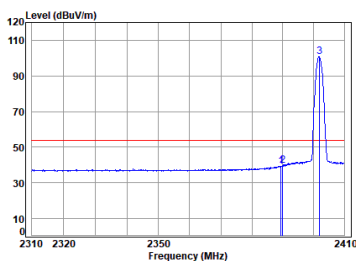
BLE_1M_TX_CH_00_Horizontal-AVG
