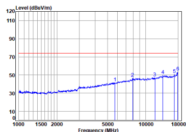
BLE_2M_TX_CH_19_Horizontal-Peak
