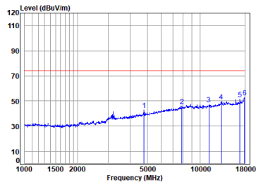
BLE_2M_TX_CH_39_Vertical-Peak
