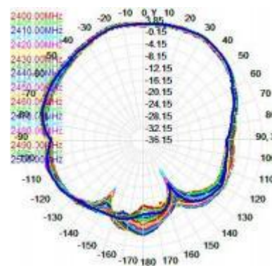
H (XY)
