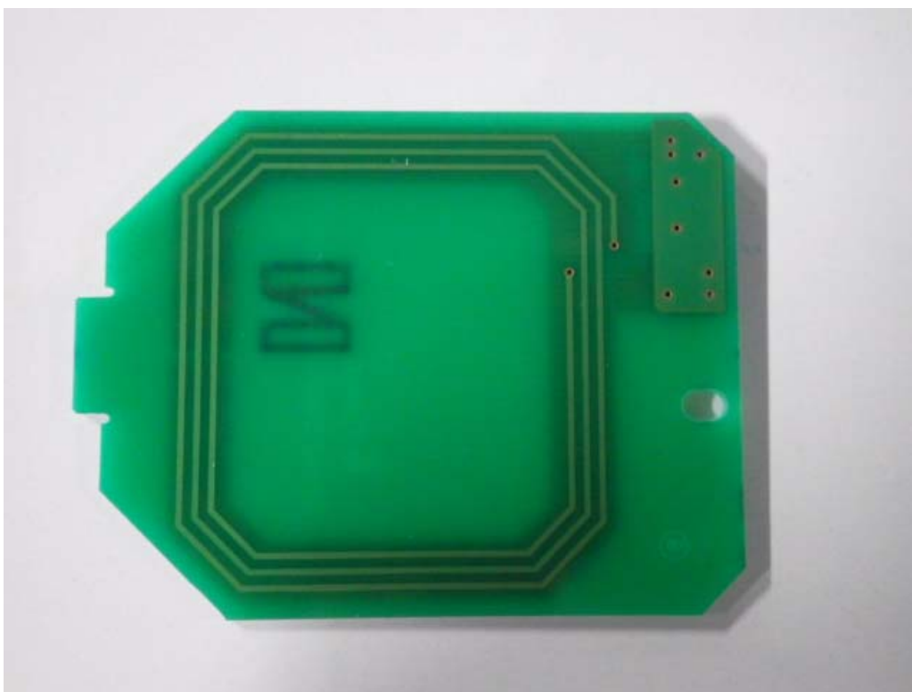
Antenna (Reverse)
