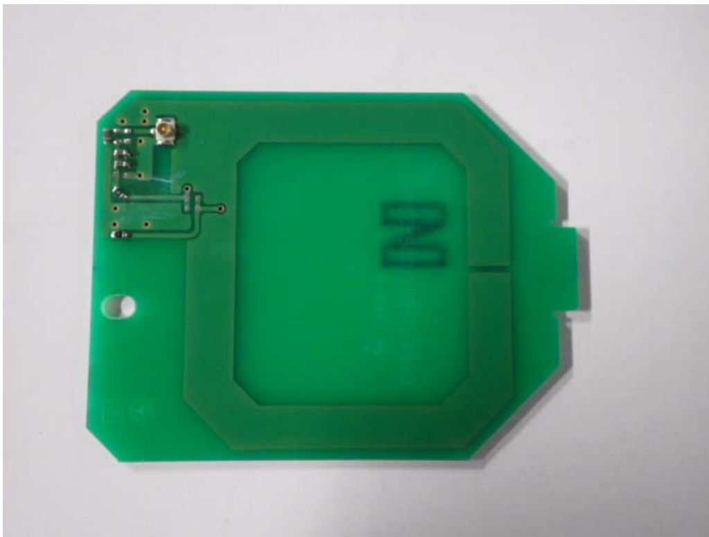
Antenna (Surface)
