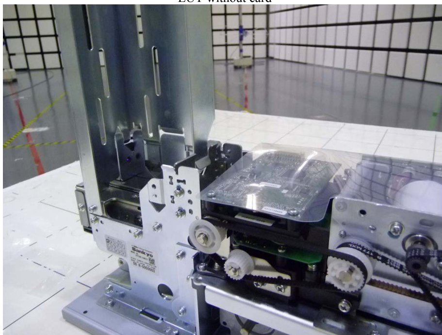
EUT without card
