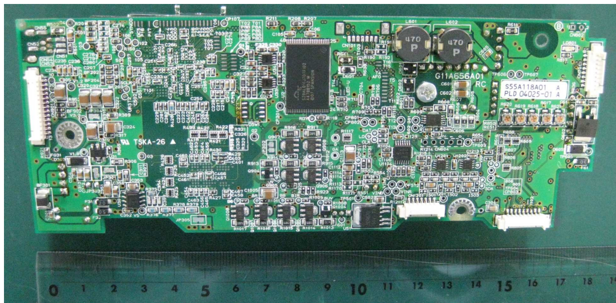
Main PCB (Surface)
