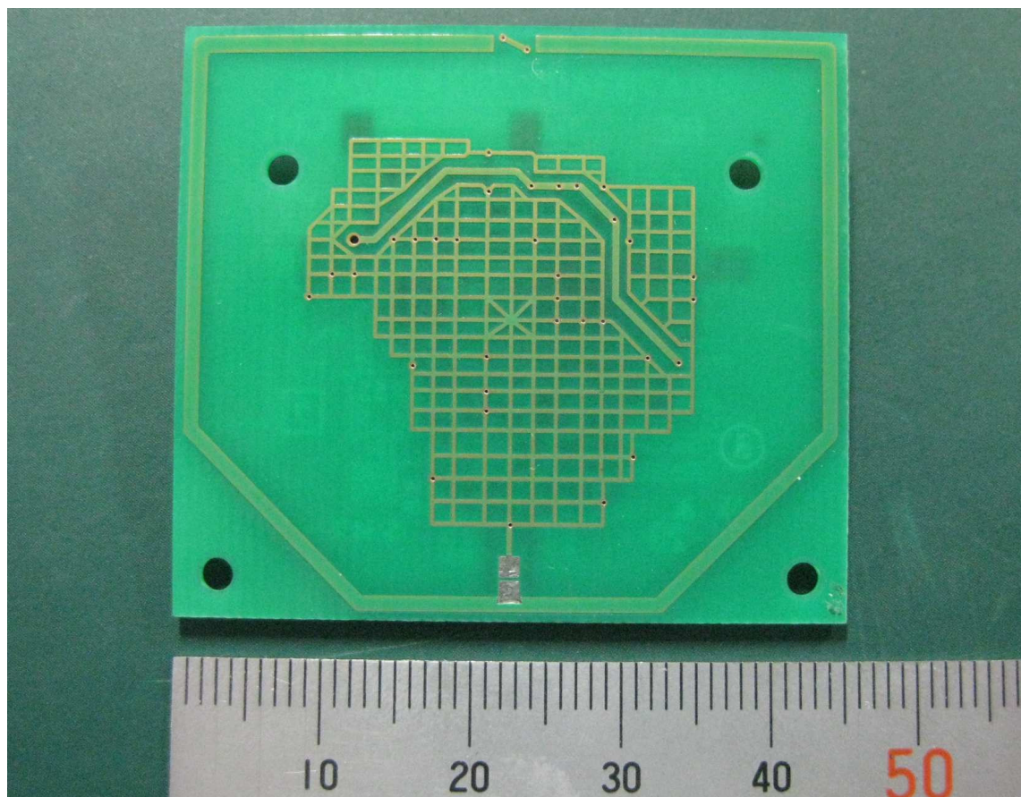
RF Circuit & Antenna Circuit Board (Back side)
