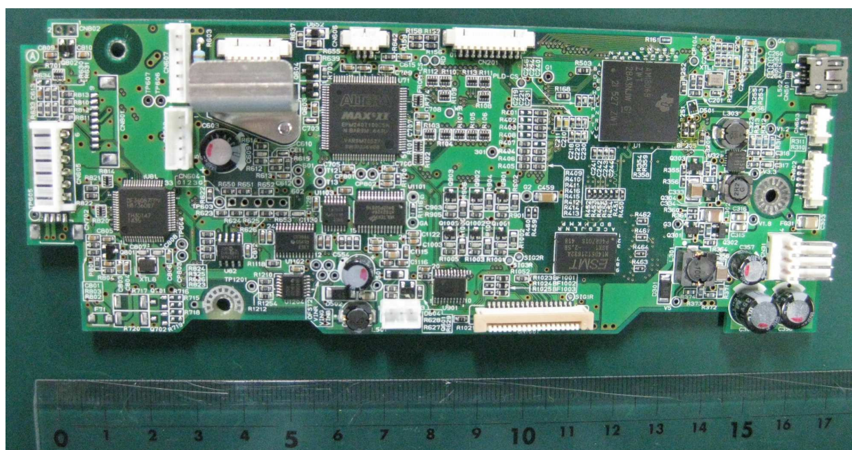
Main PCB (Back side)
