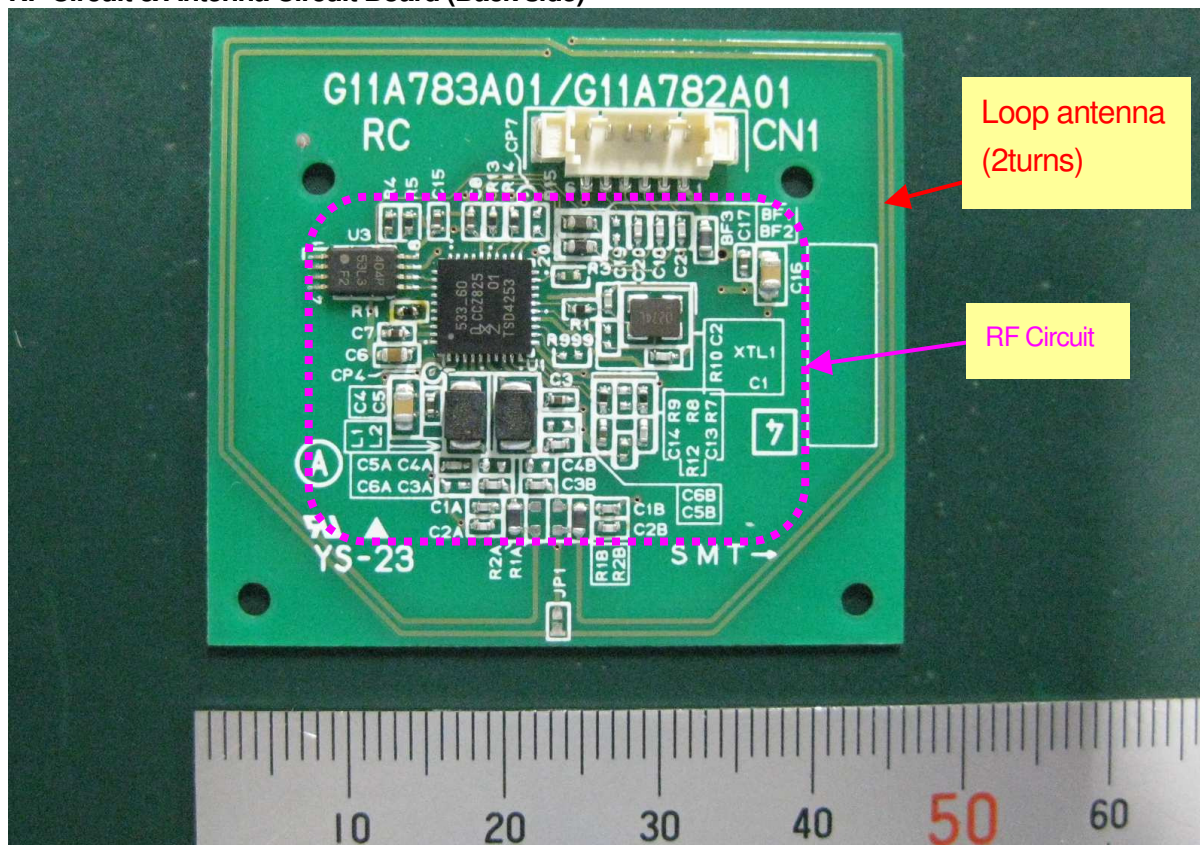
RF Circuit & Antenna Circuit Board (Back side)
