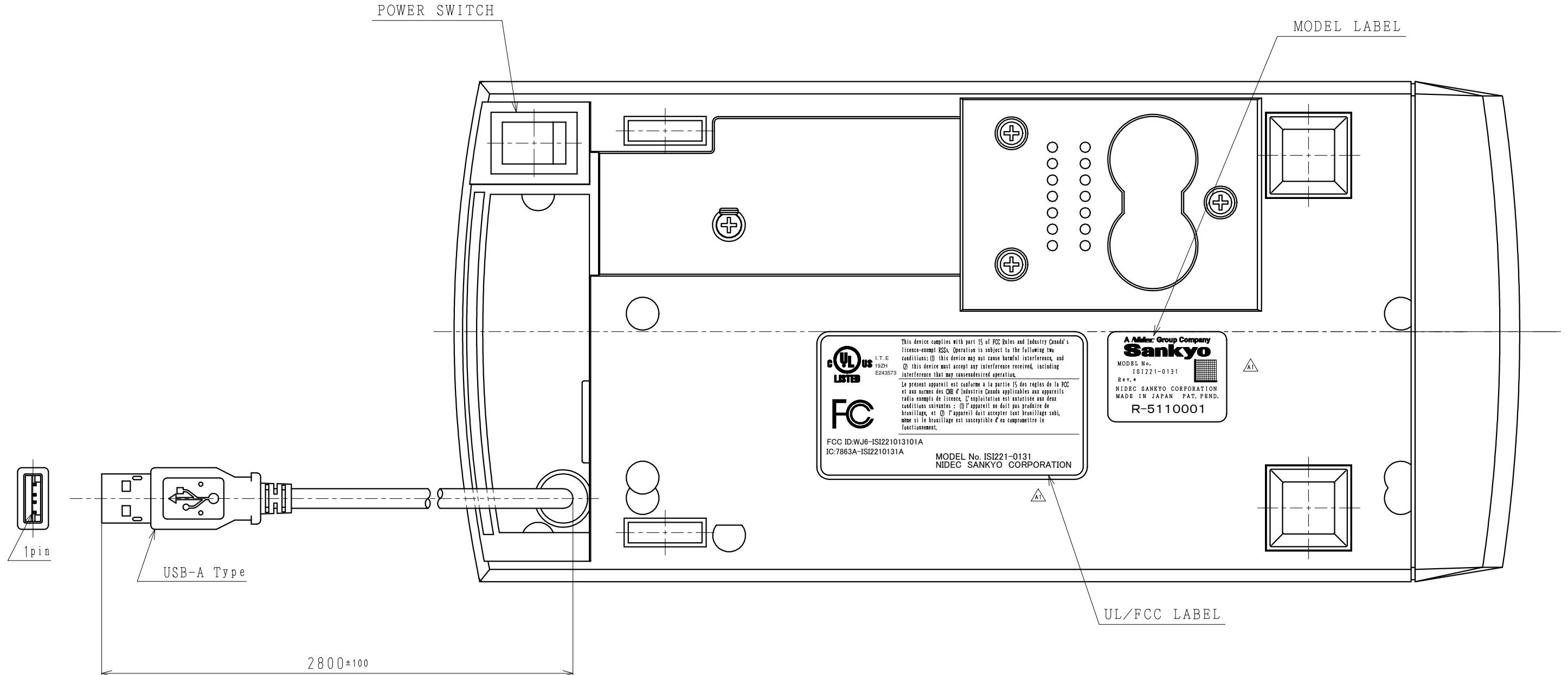
UL/FCC/IC LABEL (2/1)
