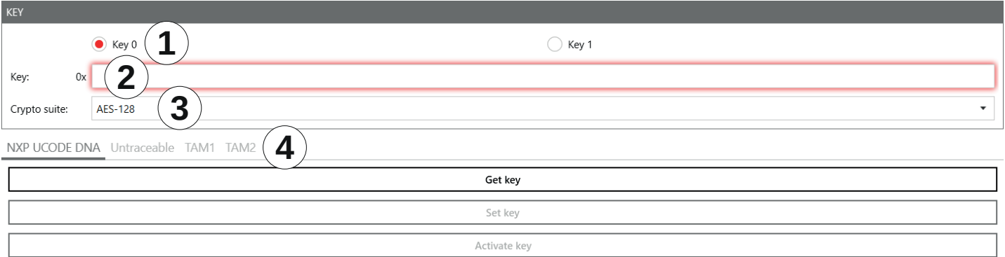
Fig. 91: Authentication: Key
