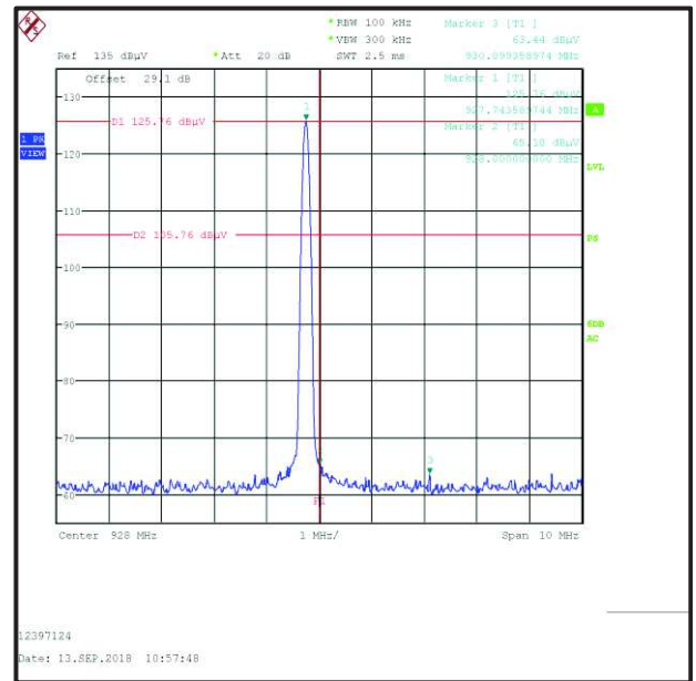
Upper Band Edge Peak Measurement
