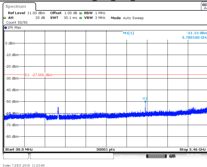
11AC40SISO_Ant1_5670_5735~40000
