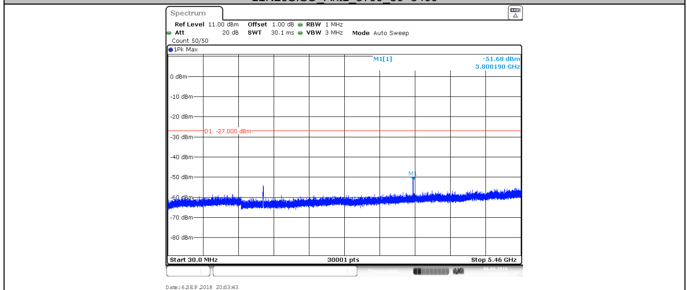
11N20SISO_Ant1_5700_5735-40000
