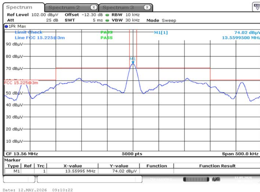
Plot 4: Spectrum mask zoomed
