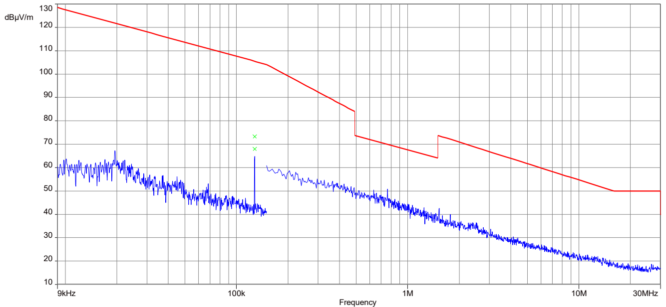
Plot 5: 9 kHz – 30 MHz, magnetic spurious emissions FCC, 127.55 kHz charging mode
