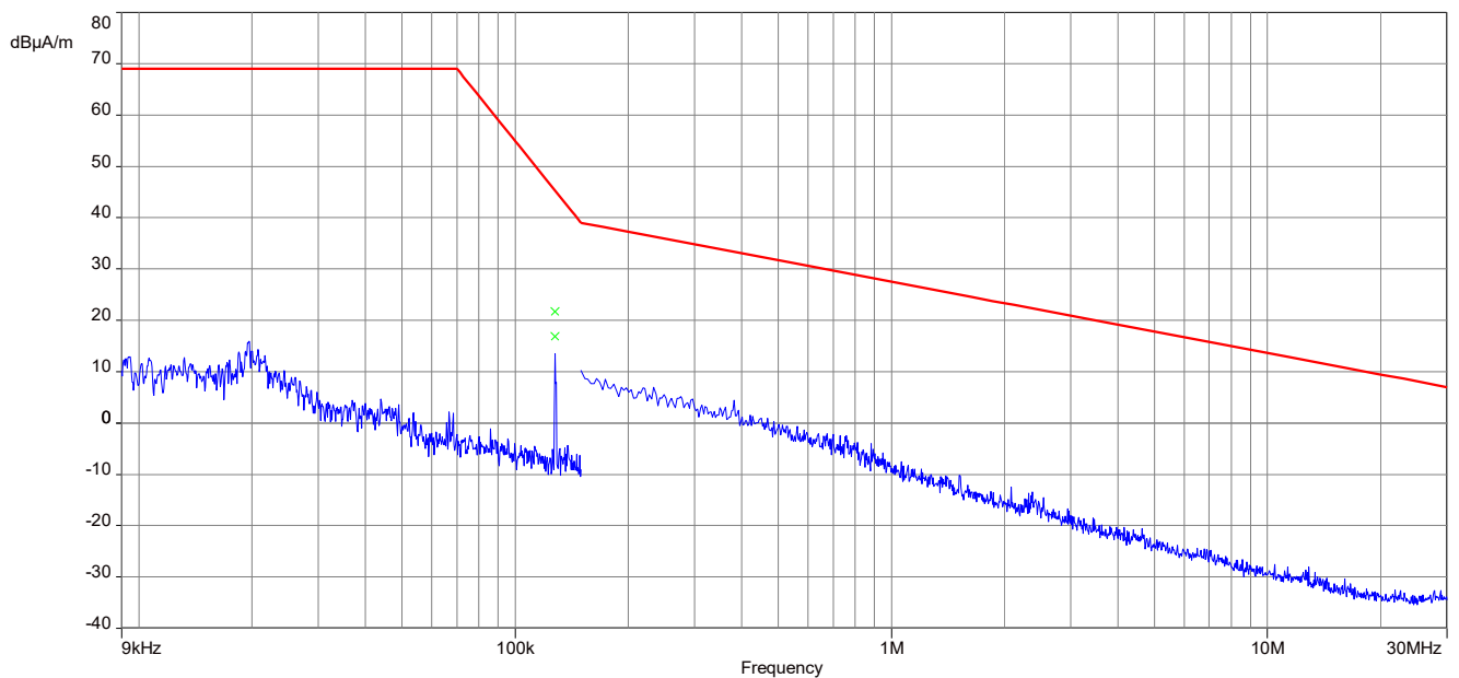
Plot 6: 9 kHz – 30 MHz, magnetic spurious emissions ISSED, 127.55 kHz charging mode
