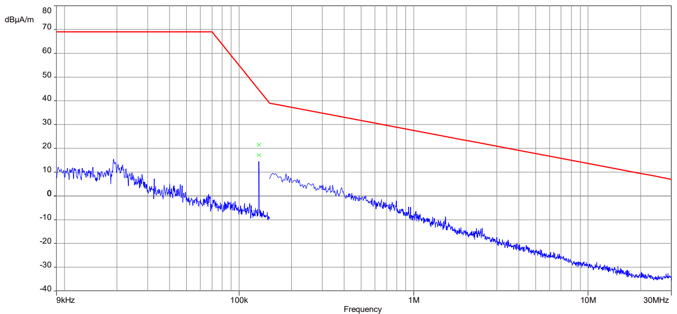
Plot 10: 9 kHz – 30 MHz, magnetic spurious emissions ISCED, 129.75 kHz charging mode
