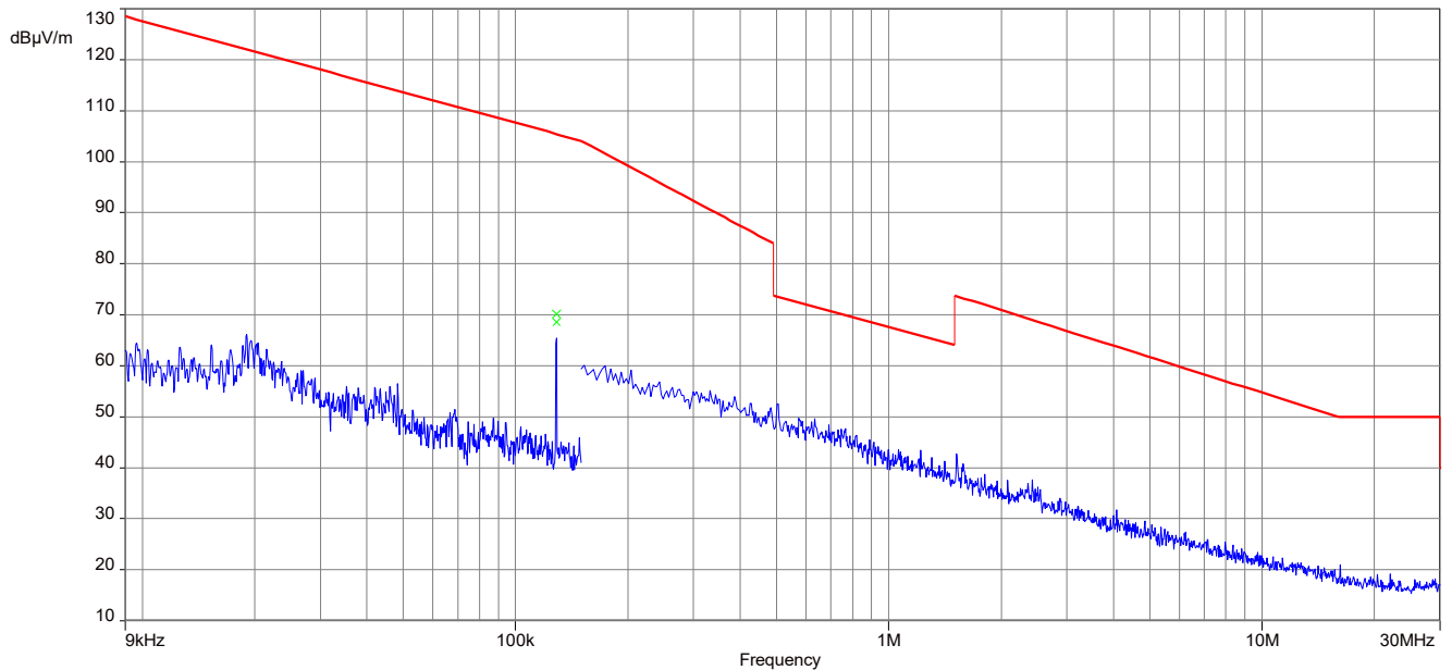
Plot 7: 9 kHz – 30 MHz, magnetic spurious emissions FCC, 128.55 kHz charging mode
