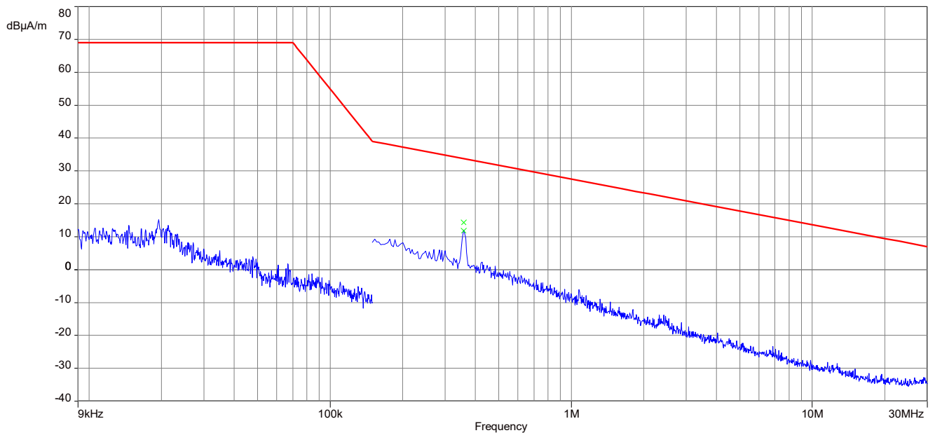
Plot 12: 9 kHz – 30 MHz, magnetic spurious emissions ISCED, 360 kHz
