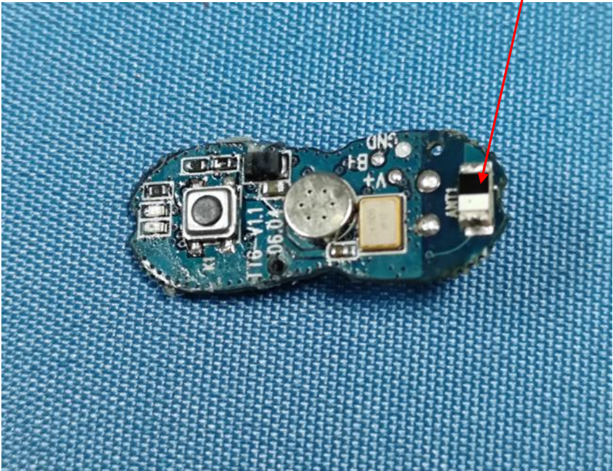
Ceramic Antenna
