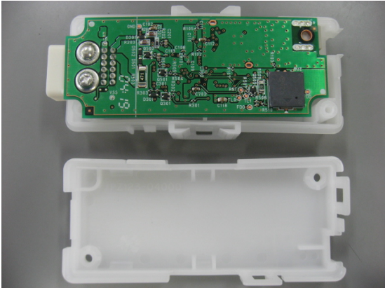
Internal Photos of Remote engine starter unit
