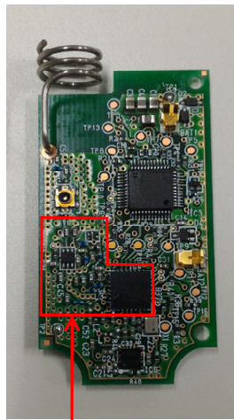
RF Block
