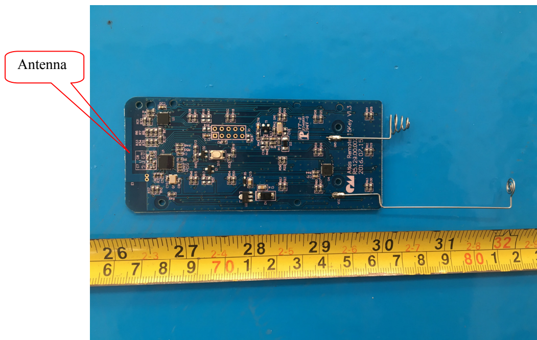
EUT –Main Board Bottom View (model number:RF369B)
