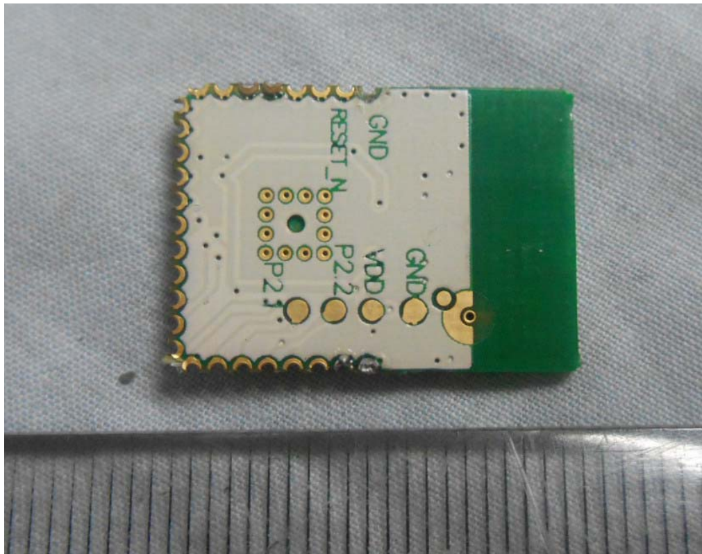
FIGURE 7 BLUETOOTH (M/N: BT-ADJUSTABLE BED) RF MODULE (BACK VIEW)
