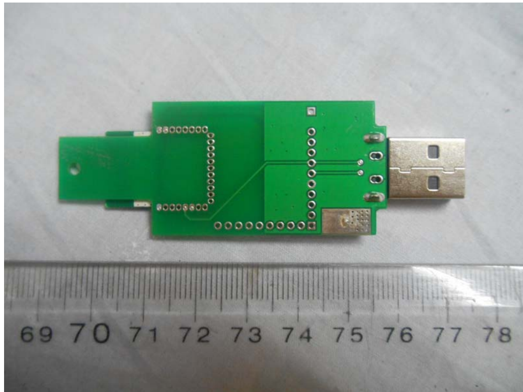
FIGURE 5 BLUETOOTH (M/N: BT-ADJUSTABLE BED) MAIN BOARD (BACK VIEW)
