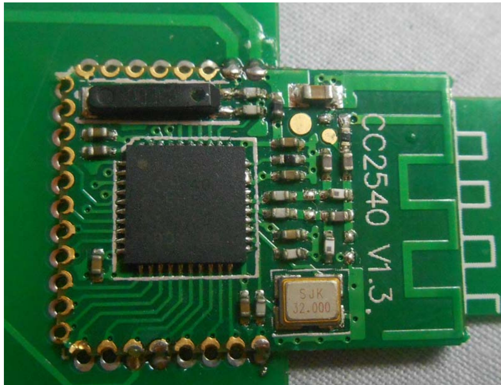
FIGURE 6 BLUETOOTH (M/N: BT-ADJUSTABLE BED) RF MODULE (FRONT VIEW)
