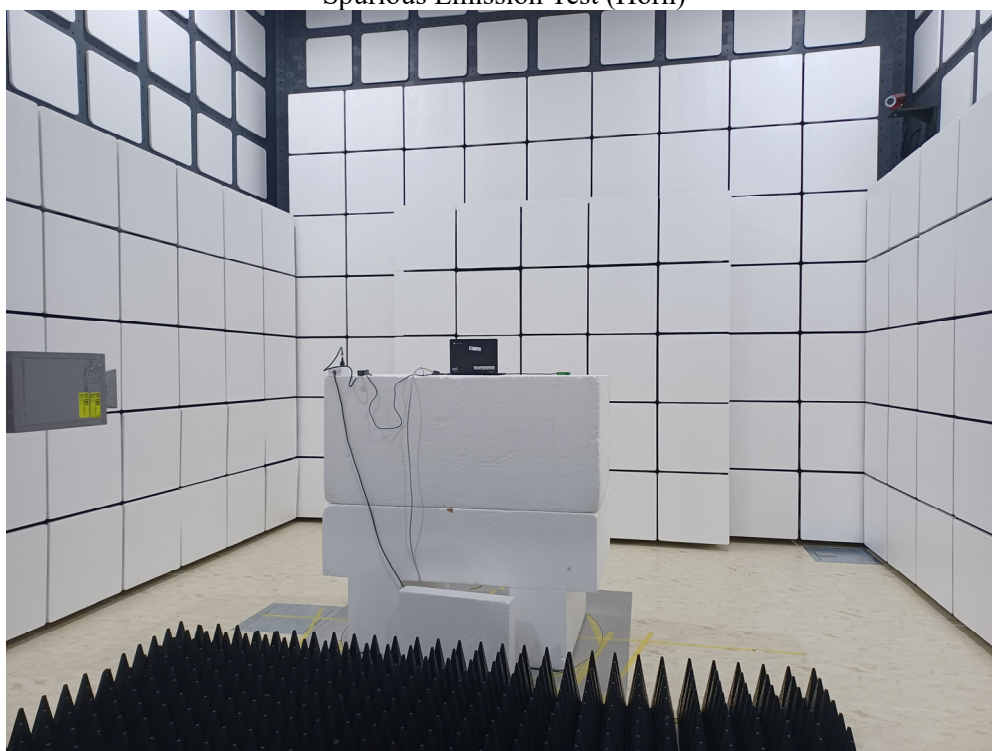
Spurious Emission Test (Horn)
