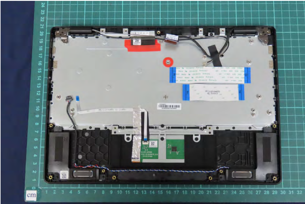
(23) EUT Photo
