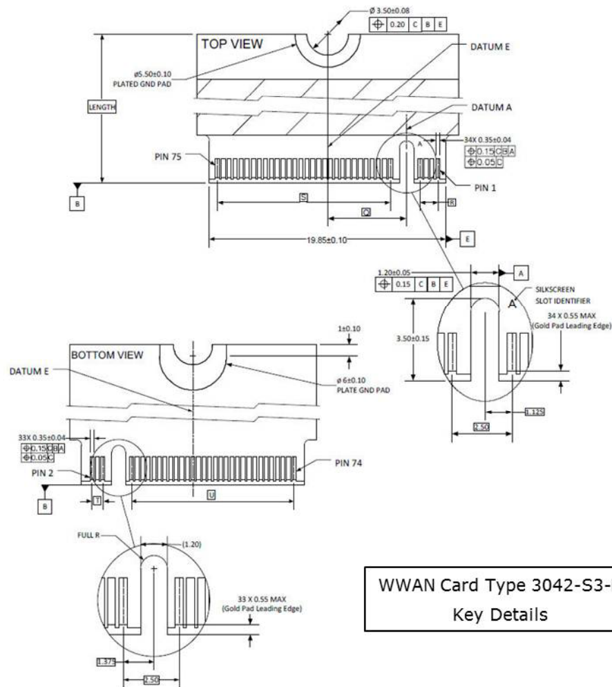
Figure 18 WWAN Card 3042 Slot Key Details
