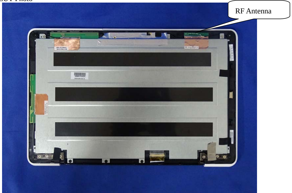
(25) EUT Photo
