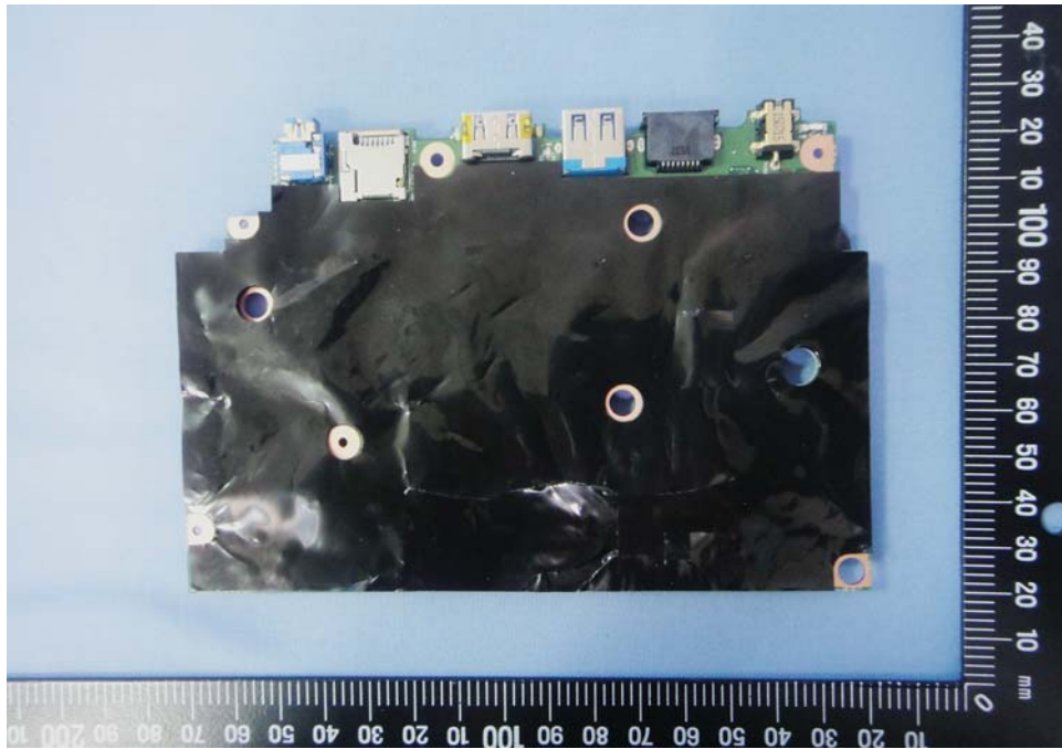
(20)EUT Photo
