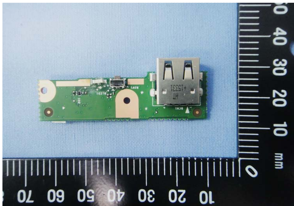
(28)EUT Photo
