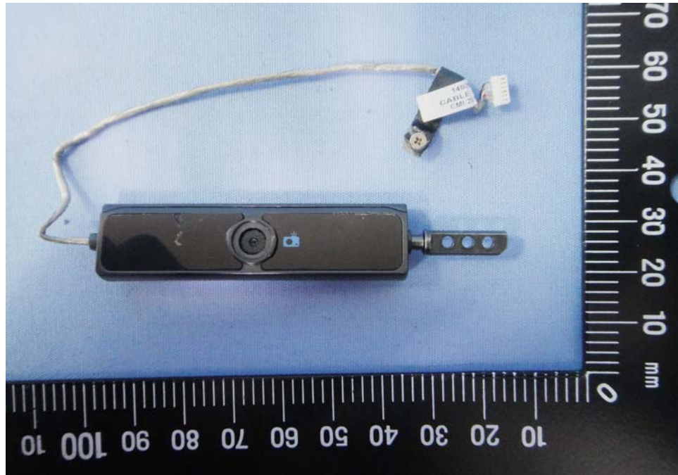
(42)EUT Photo
