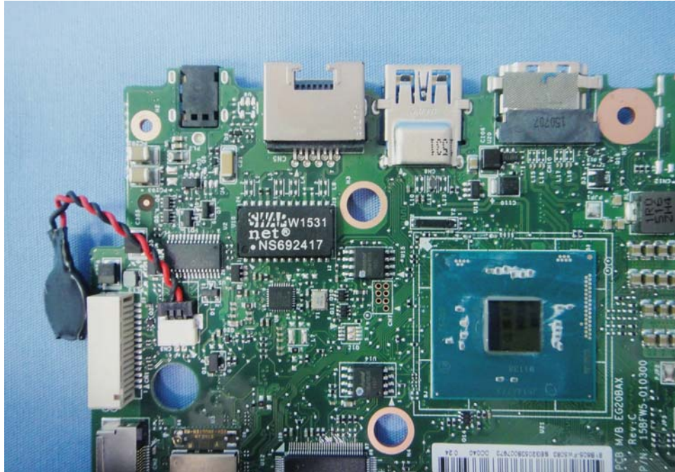
(16)EUT Photo
