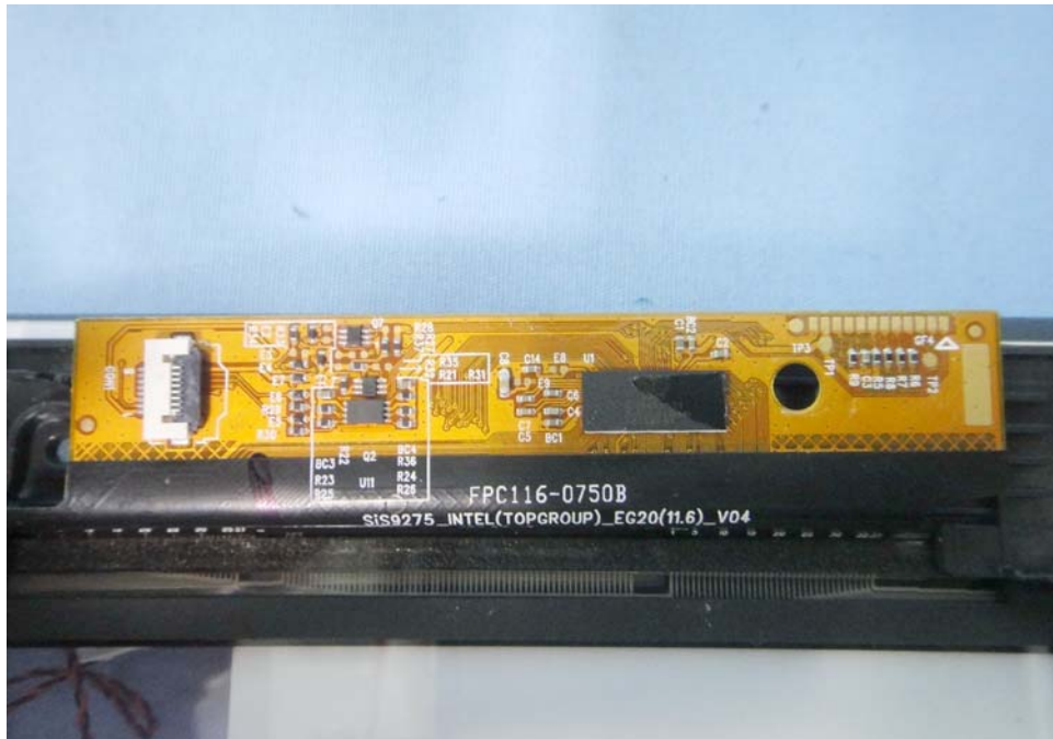
(48)EUT Photo
