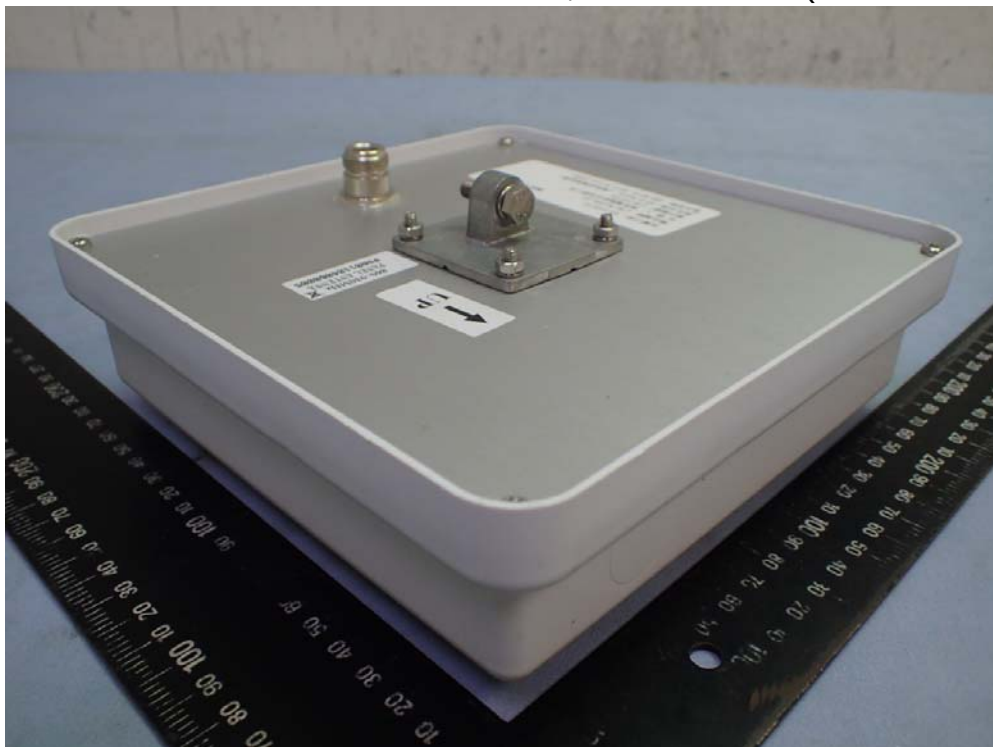
Figure 6 Panel Antenna, General View (Back & Side View)
